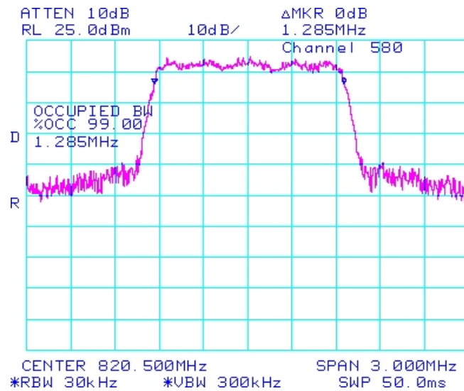
Figure 1-8b: Occupied Bandwidth, Cellular Middle Channel
