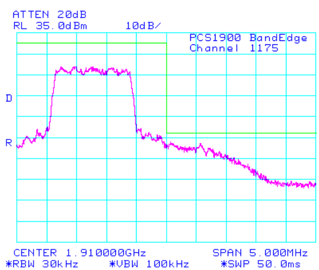
Figure 1-24b: PCS High Channel Mask
