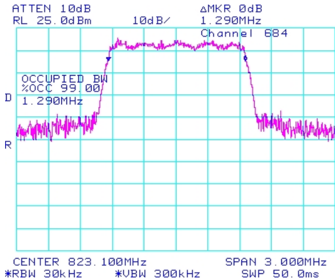
Figure 1-9b: Occupied Bandwidth, Cellular High Channel
