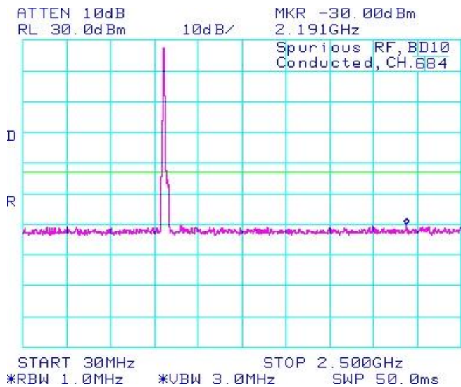
Figure 9-5b: Cellular, Spurious Conducted Emissions, High Channel
