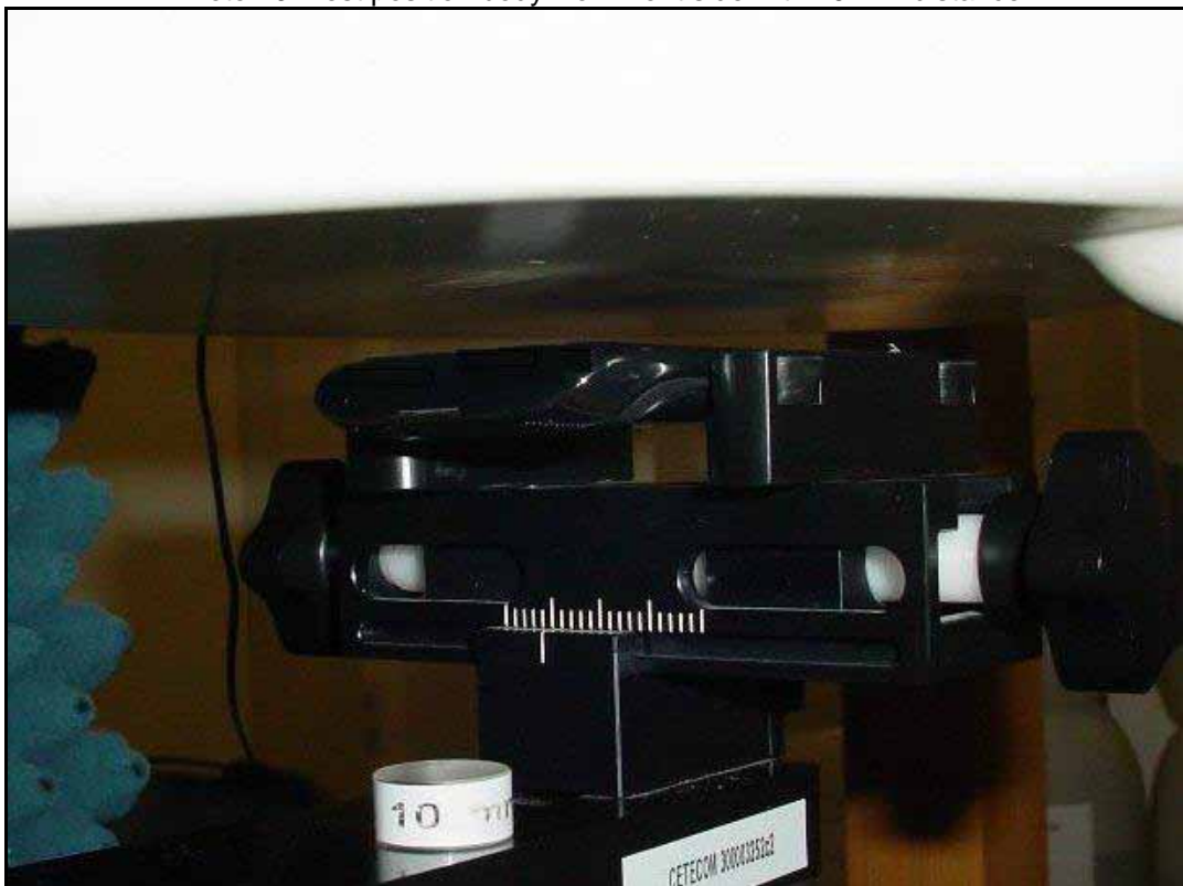
Photo 10: Test position body worn front side with 10 mm distance
