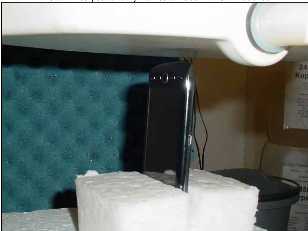
Photo 14: Test position body worn bottom side with 10 mm distance
