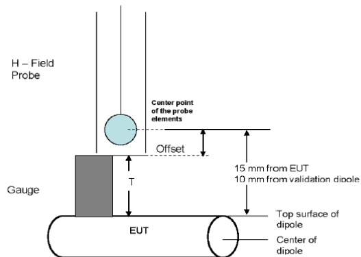
H-Field Probe (H3DV6)
