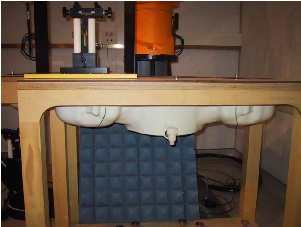
Figure 8.1. DASYS system with absorbing material
