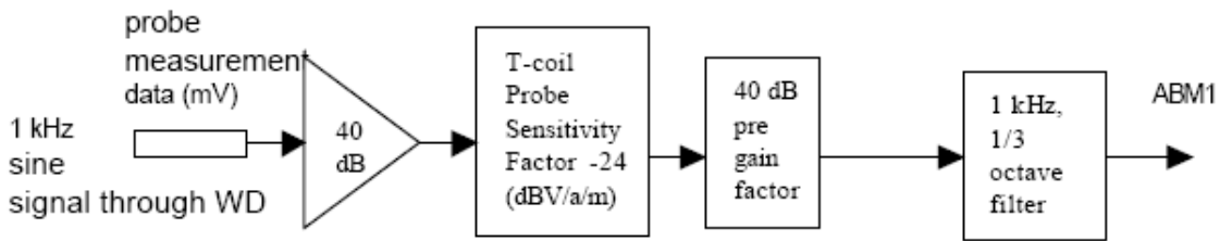
Figure 6.2. ABM1 block diagram
