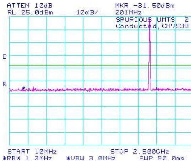
Figure 1-11b: UMTS band 2, Spurious Conducted Emissions, High Channel
