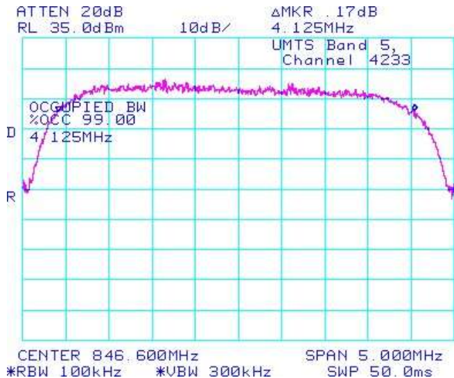
Figure 1-43b: Occupied Bandwidth, UMTS band 5 High Channel
