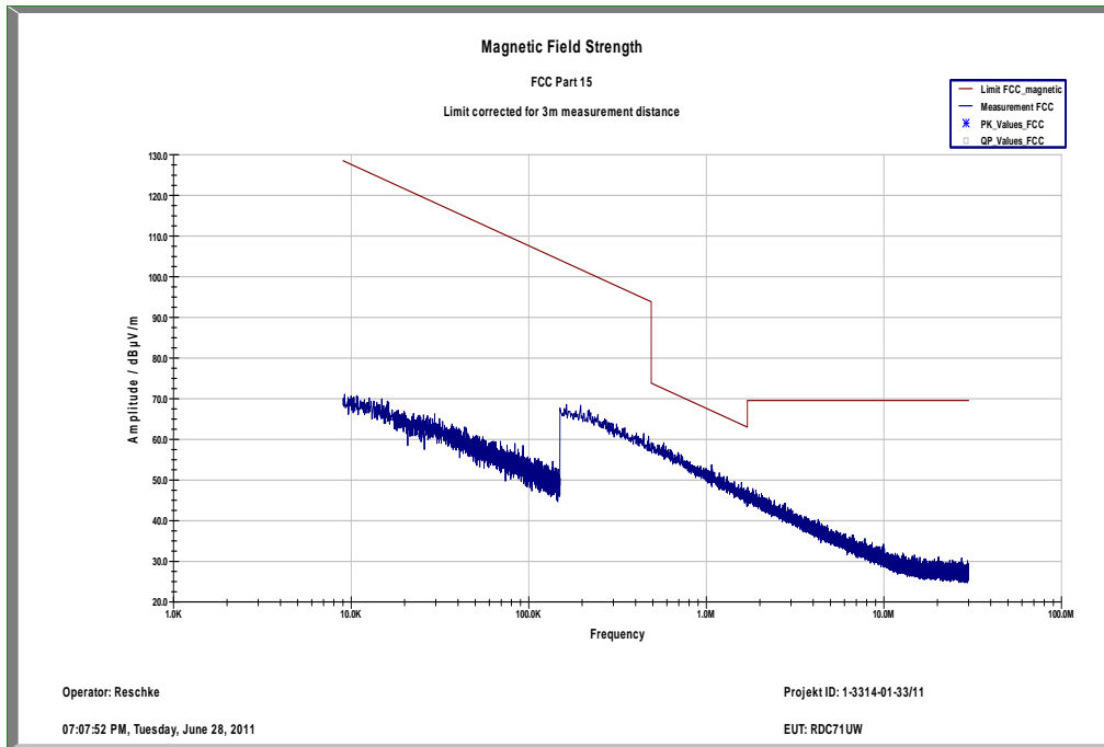
Plot 1: Channel 9262 (Traffic mode up to 30 MHz)
