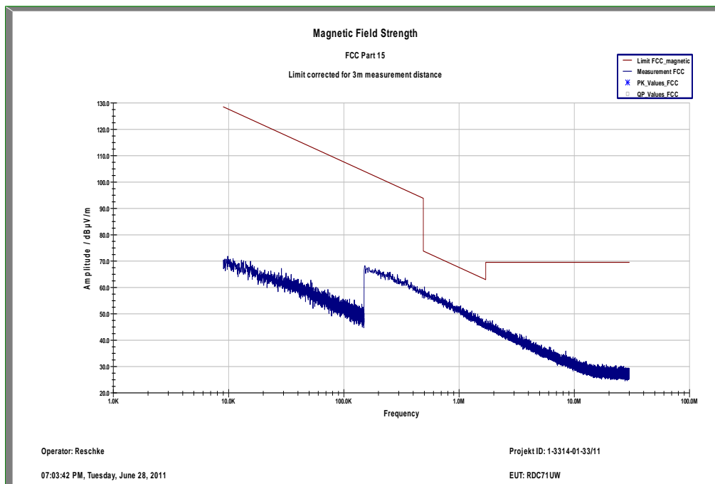
Plot 15: Channel 9538 (Traffic mode up to 30 MHz)
