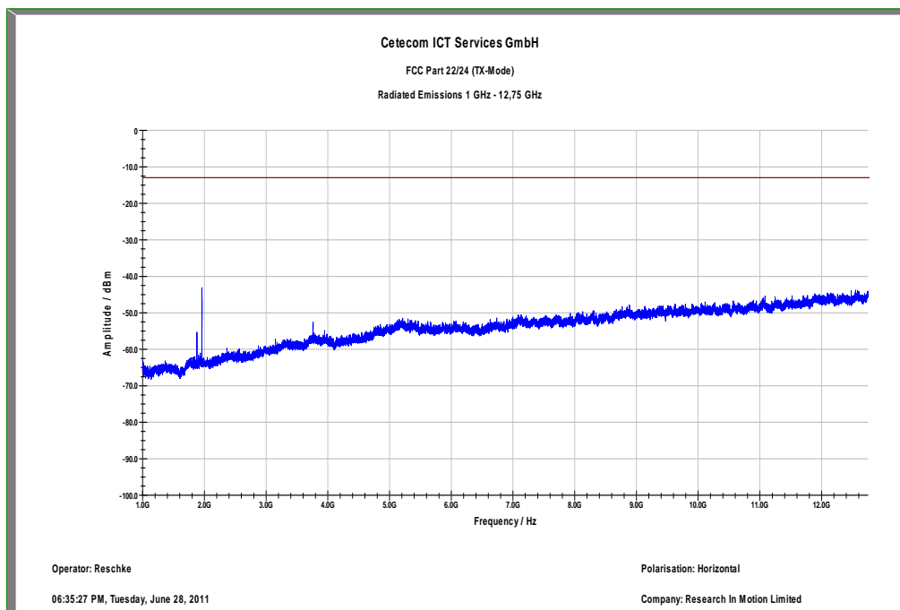
Plot 14: Channel 9400 (1 GHz – 12.75 GHz) – horizontal
