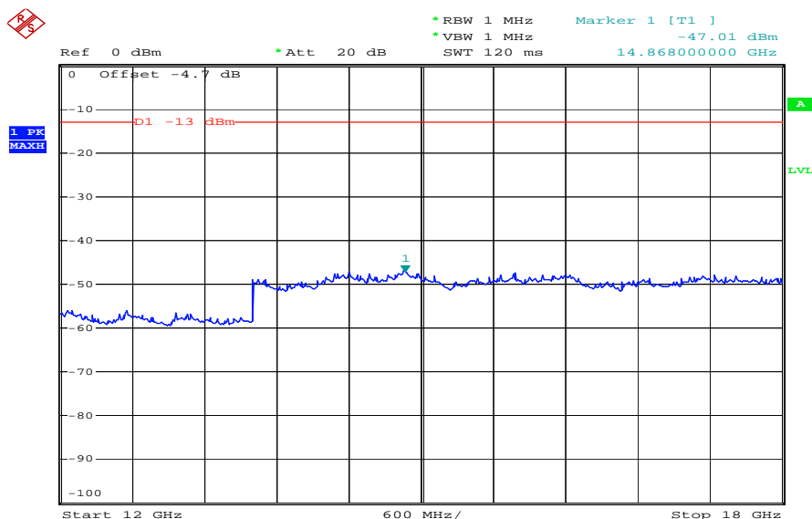
Plot 18: Channel 9538 (12 GHz - 18 GHz) – vertical/horizontal (max hold)
