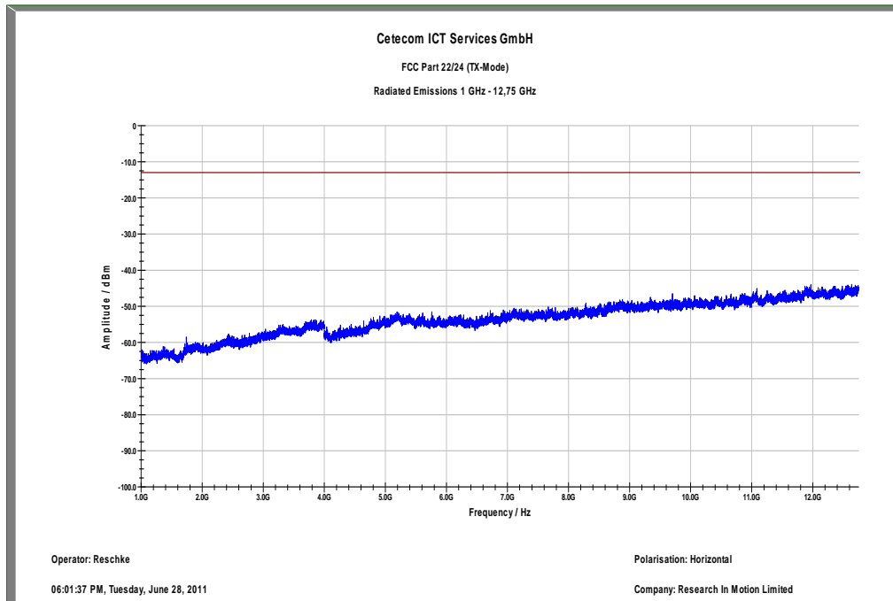
Plot 5: Channel 4132 (1 GHz – 12.75 GHz) – horizontal
