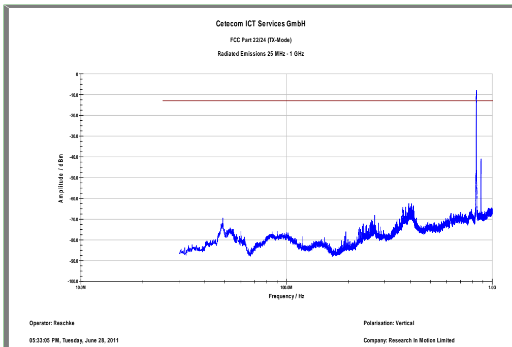
Plot 7: Channel 4180 (30 MHz - 1 GHz) – vertical
