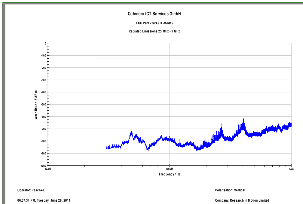
Plot 9: Channel 9400 (30 MHz - 1 GHz) – vertical
