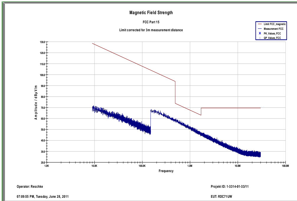
Plot 1: Channel 4132 (Traffic mode up to 30 MHz)
