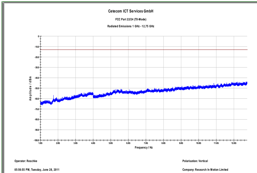
Plot 3: Channel 4132 (1 GHz – 12.75 GHz) – vertical
