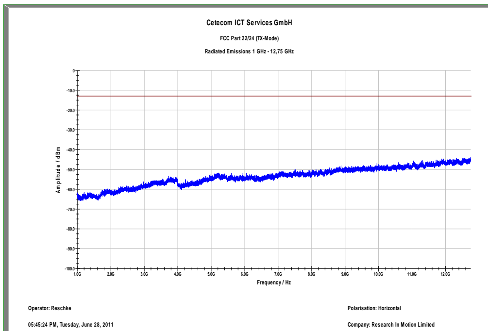
Plot 15: Channel 4233 (1 GHz – 12.75 GHz) – horizontal
