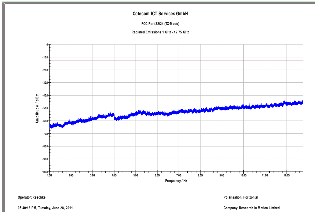
Plot 10: Channel 4180 (1 GHz – 12.75 GHz) – horizontal
