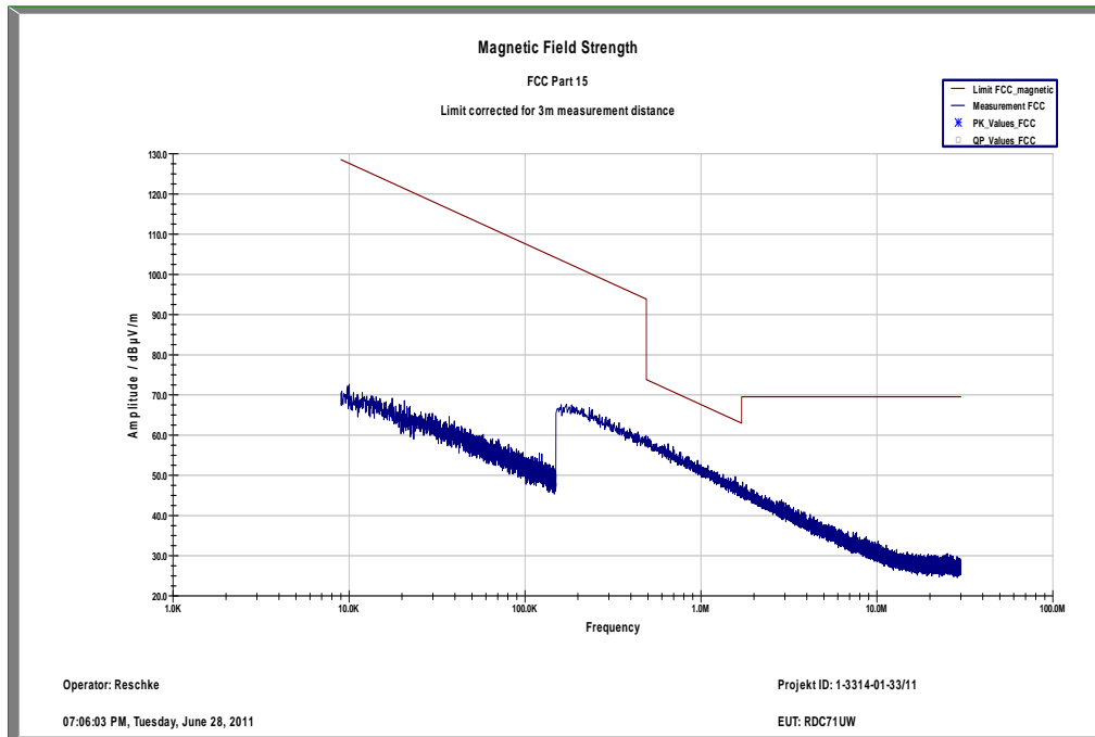
Plot 8: Channel 9400 (Traffic mode up to 30 MHz)
