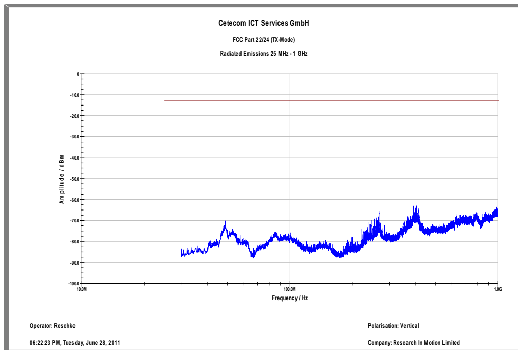
Plot 2: Channel 9262 (30 MHz - 1 GHz) – vertical
