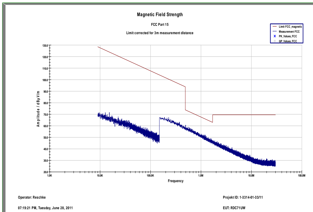
Plot 11: Channel 4233 (Traffic mode up to 30 MHz)
