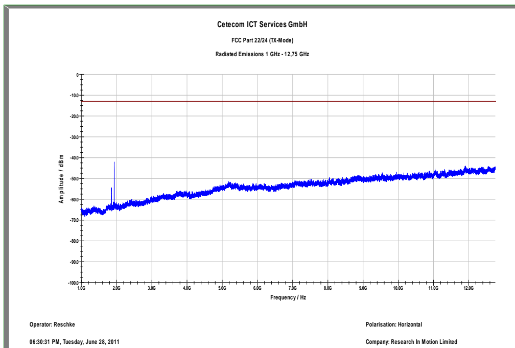
Plot 7: Channel 9262 (1 GHz – 12.75 GHz) – horizontal
