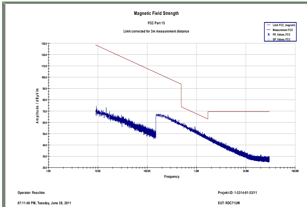
Plot 6: Channel 4180 (Traffic mode up to 30 MHz)
