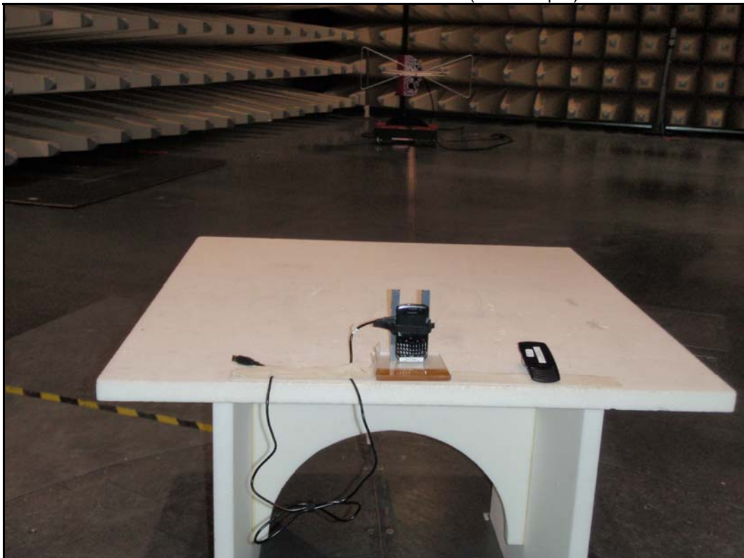
Photo 2: radiated emission < 1 GHz (Set 1 / Op 1)
