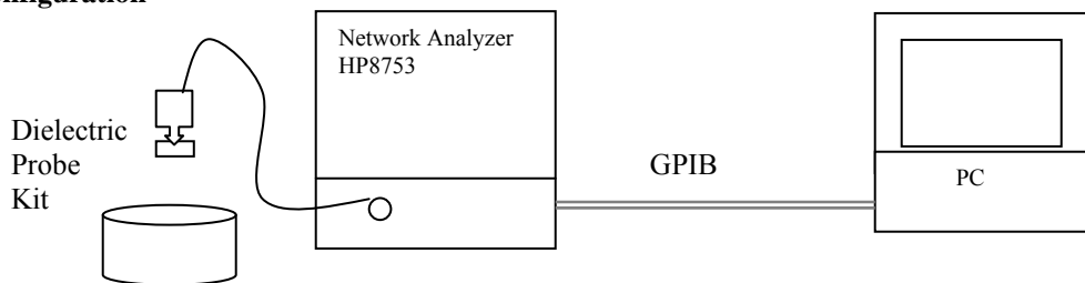
Figure 6.2.1 Test configuration
