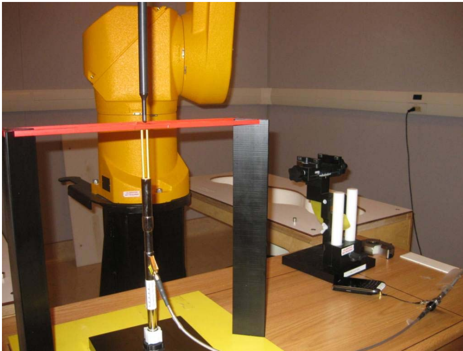
Figure 2 – Dipole Validation & Probe Modulation Factor measurement setup
