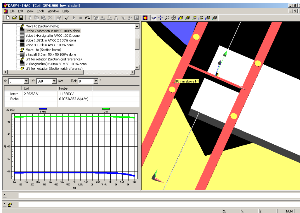
Figure 6.1. DASY4 ABM probe calibration
