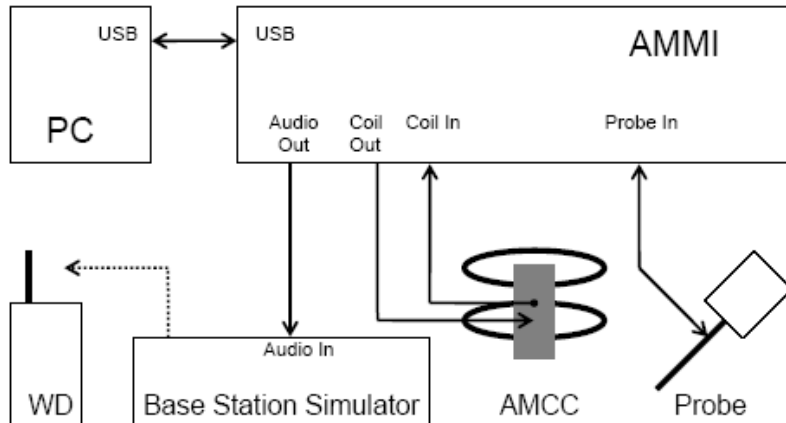
Figure 5.10.1. T-Coil set up cabling
