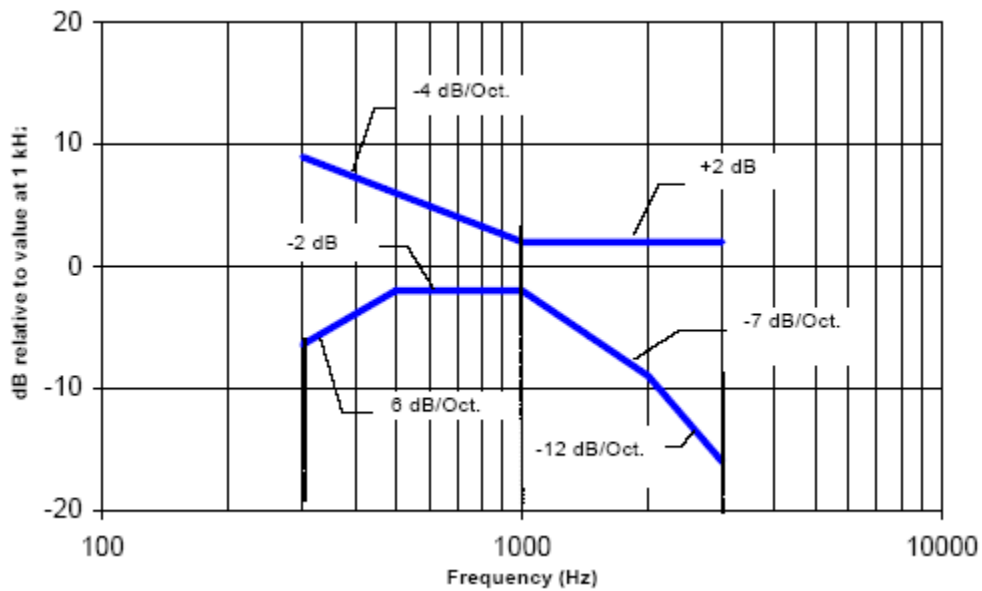
Figure 6.5.3. Magnetic field frequency response for WDs with a field that exceeds -15 dB(A/m) at 1 kHz
