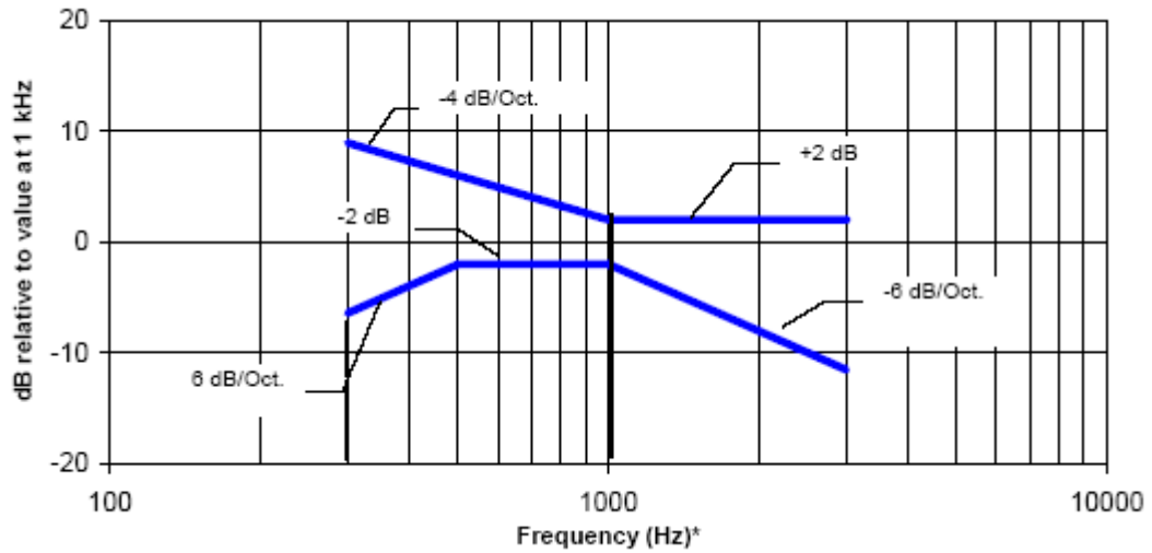
Figure 6.5.2. Magnetic field frequency response for WDs with a field that is \leq -15 dB (A/m) at 1 kHz
