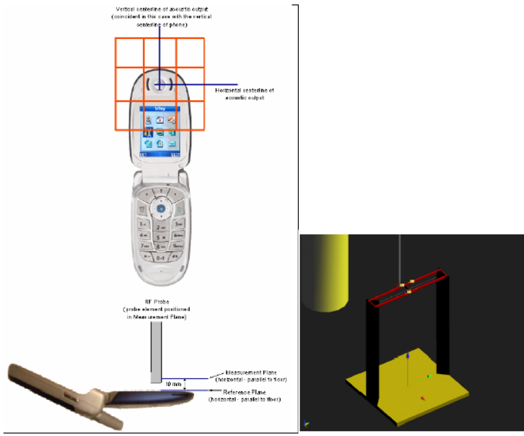
Figure 5.2.1 WD reference plane for RF emission measurements Figure 5.2.2: HAC Phantom/Test Arch
