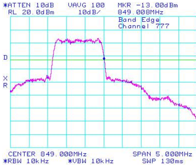
Figure 11-21b: Cellular Loopback, High Channel Mask
