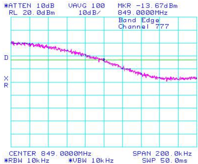
Figure 1-22b: Cellular Loopback, High Channel Mask
