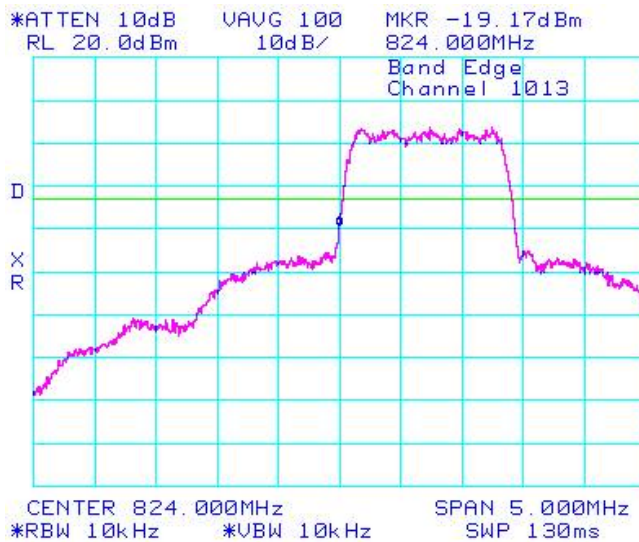
Figure 1-19b: Cellular Loopback, Low Channel Mask
