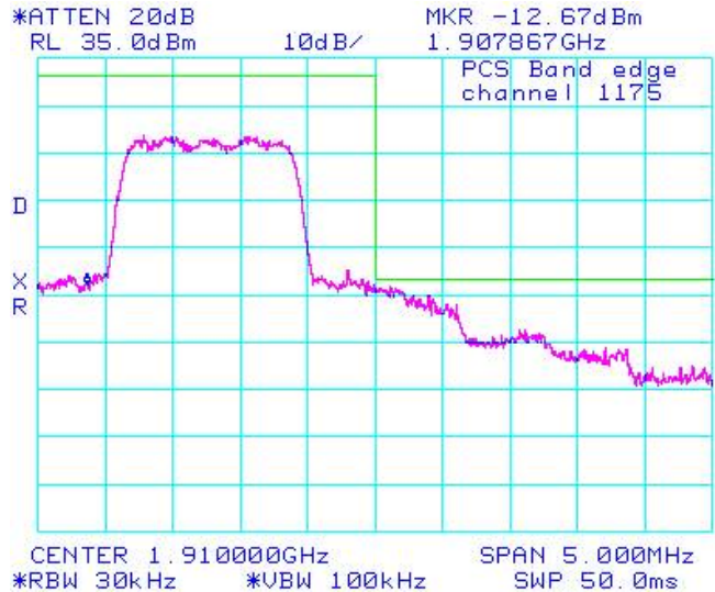
Figure 1-24b: PCS Loopback, High Channel Mask
