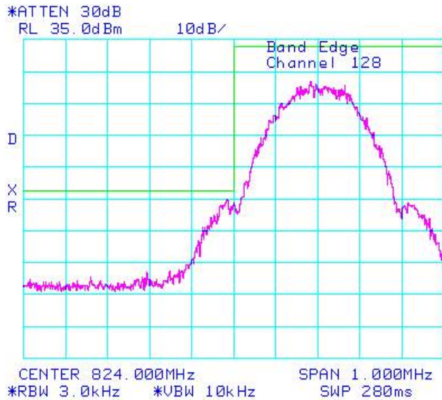
Figure 1-35a: GSM850 Band, Low Channel Mask in EDGE mode
