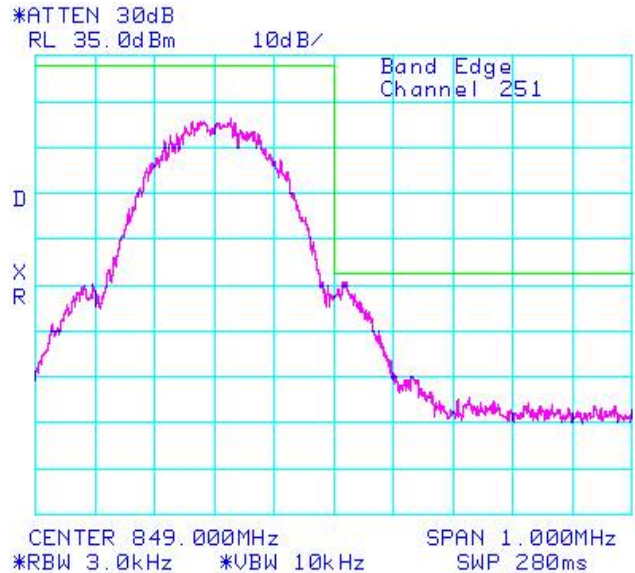
Figure 1-36a: GSM850 Band, High Channel Mask in EDGE mode
