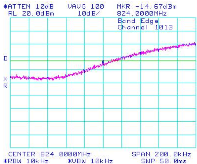
Figure 1-20b: Cellular Loopback, Low Channel Mask
