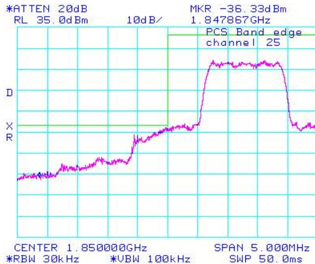
Figure 1-23b: PCS Loopback, Low Channel Mask
