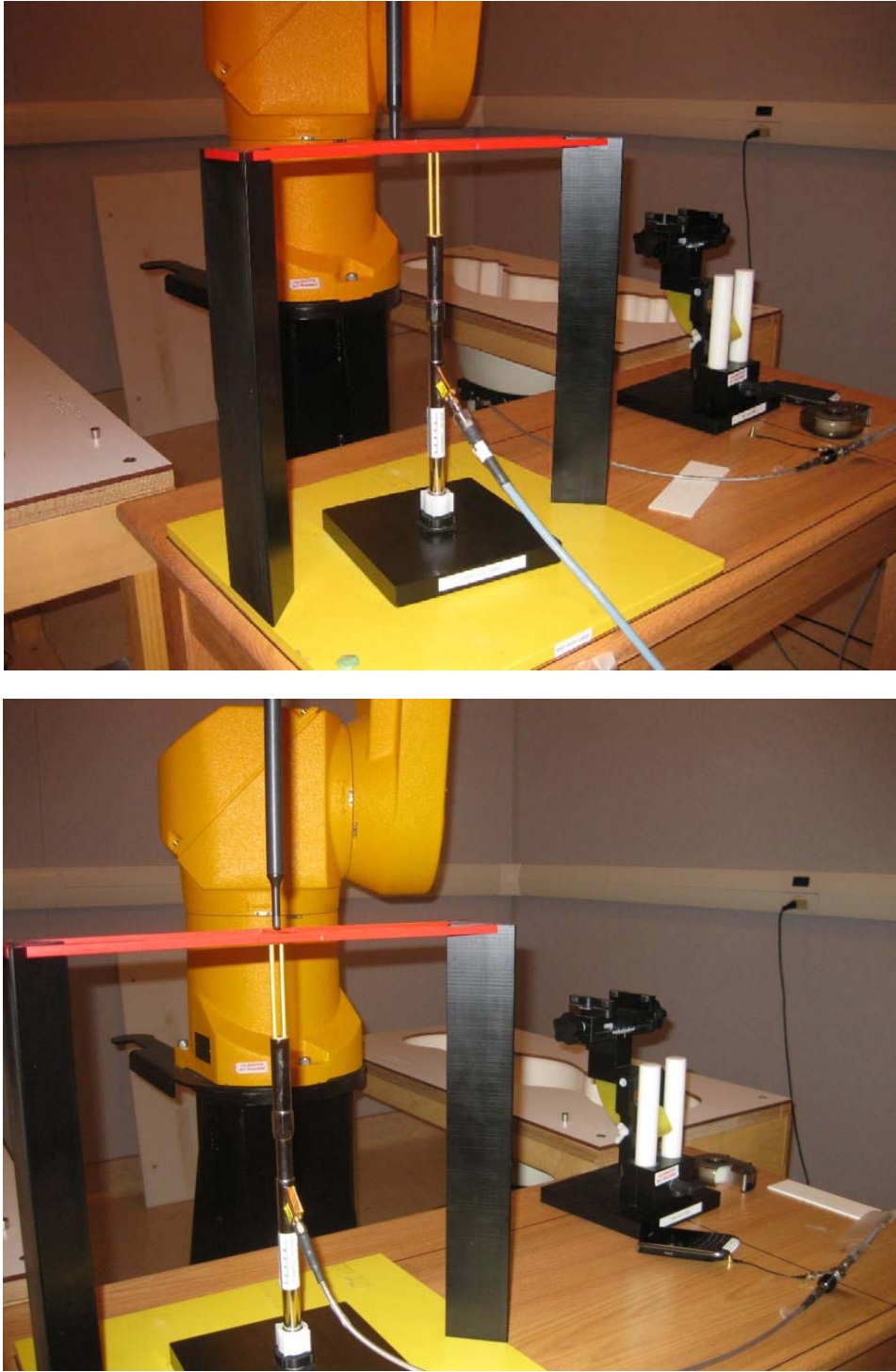
Figure 2 – Dipole Validation & Probe Modulation Factor measurement setup
