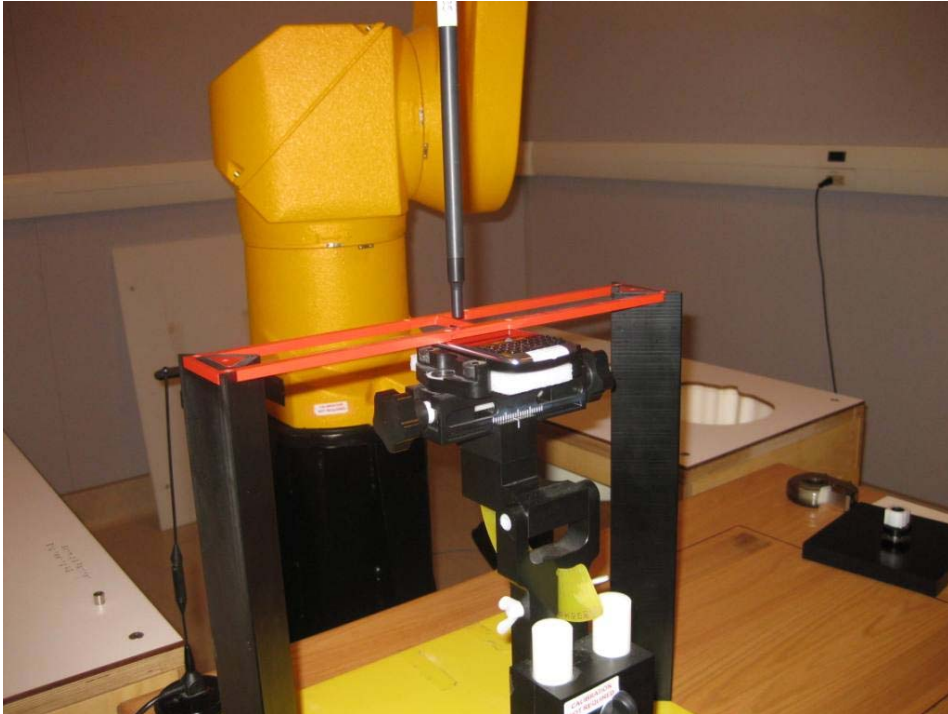
Figure 3 – HAC RF emissions test setup
