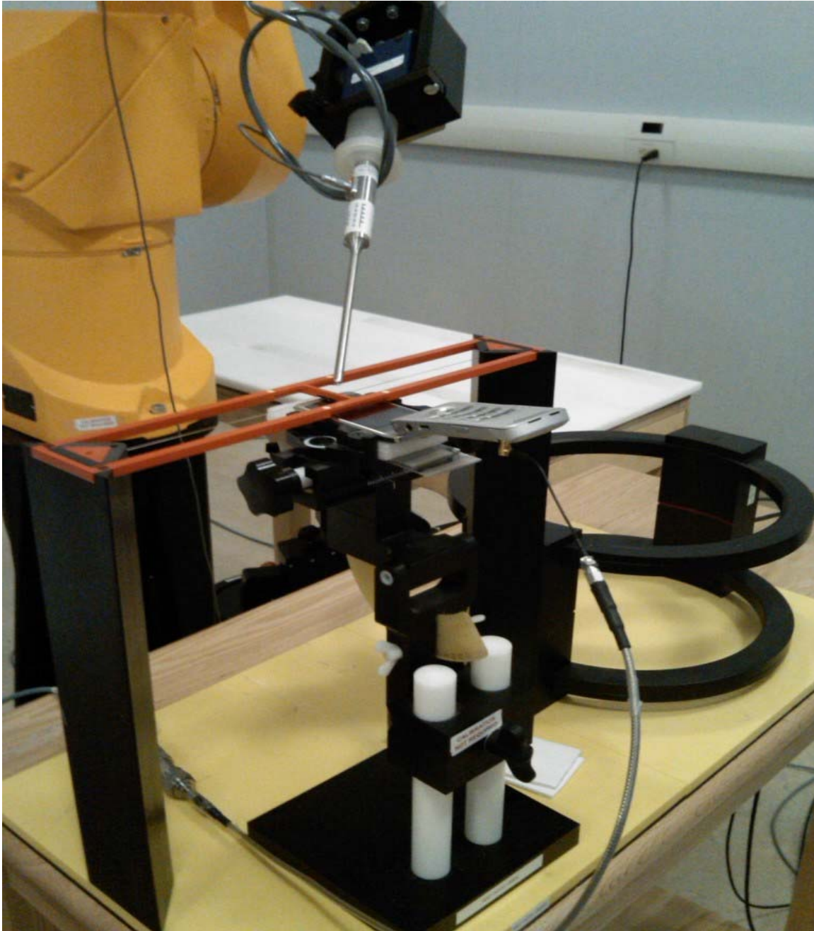
Figure E4: Audio Band Magnetic (ABM) T-Coil measurement setup
