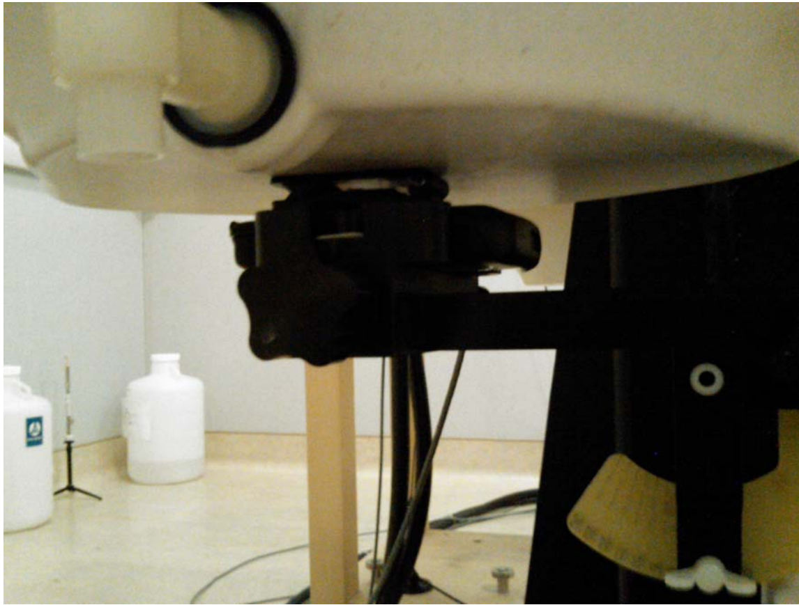
Figure E10. Body-worn configuration (Plastic Holster, front facing phantom)
