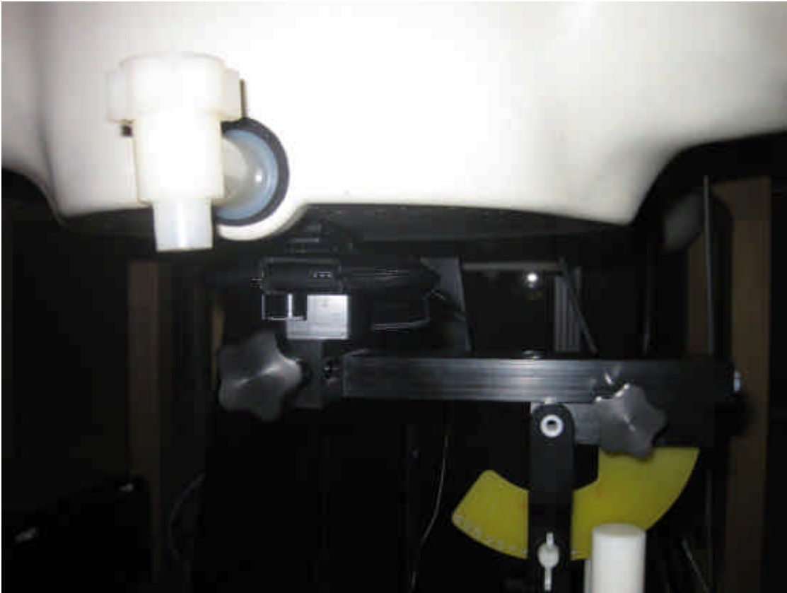
Figure E11. Body-worn configuration (Horizontal Holster, headset, back facing phantom)
