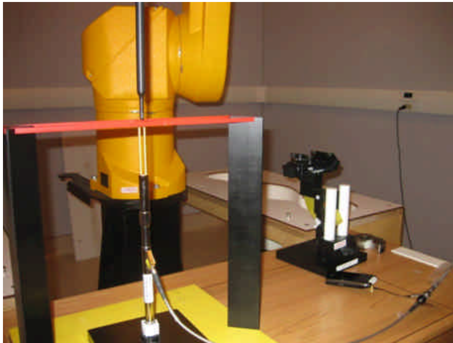
Figure 3 – Dipole Validation & Probe Modulation Factor measurement setup
