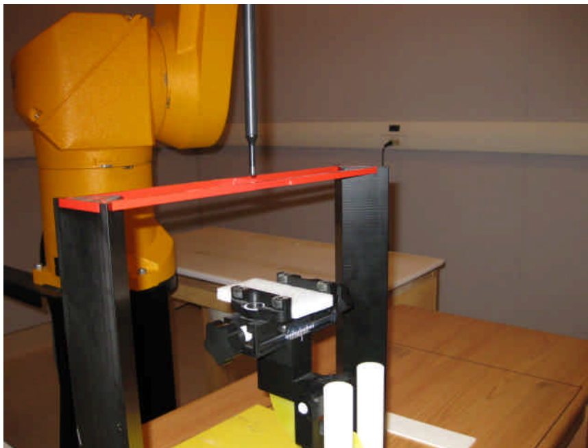
Figure 2 – RF Ambient Noise measurement setup
