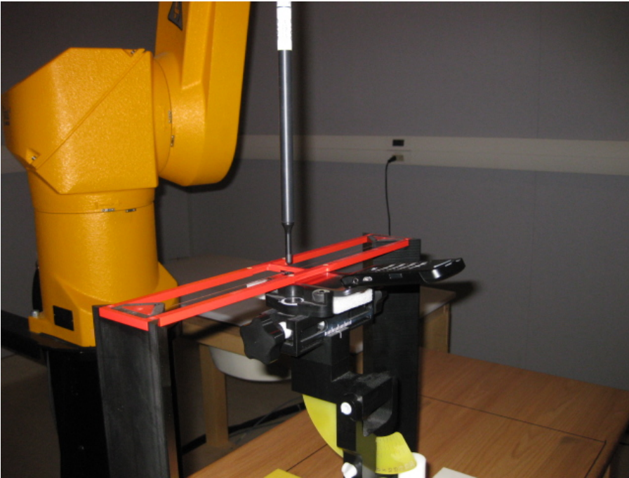
Figure 4 – HAC RF emissions test setup
