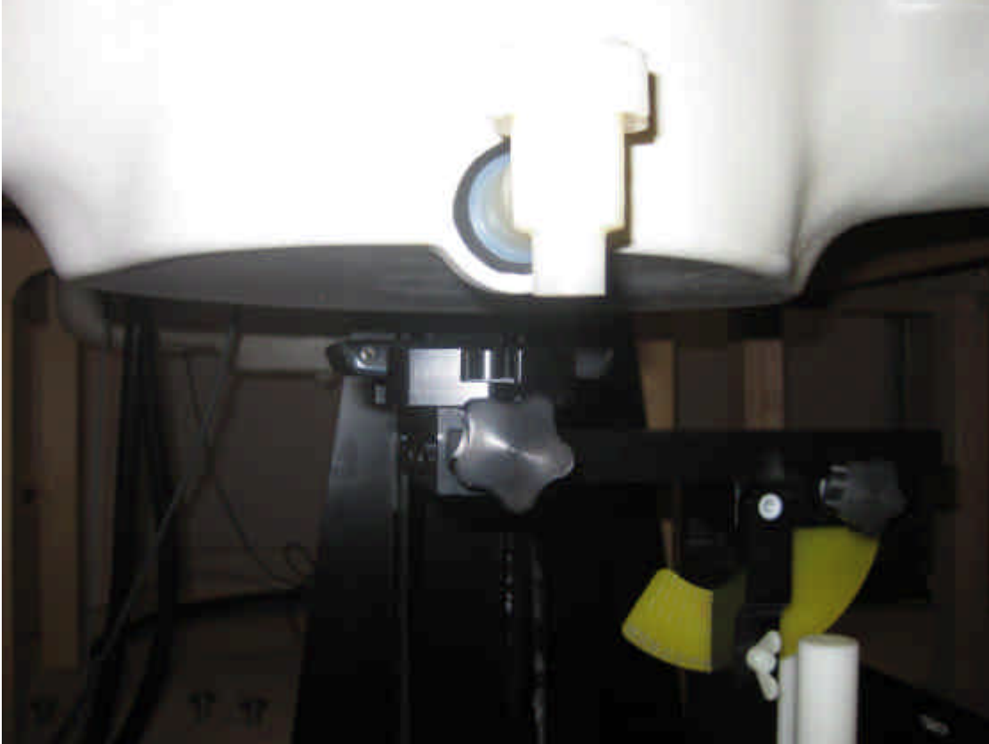
Figure E10. Body-worn configuration (No Holster, 25 mm away, back facing phantom)
