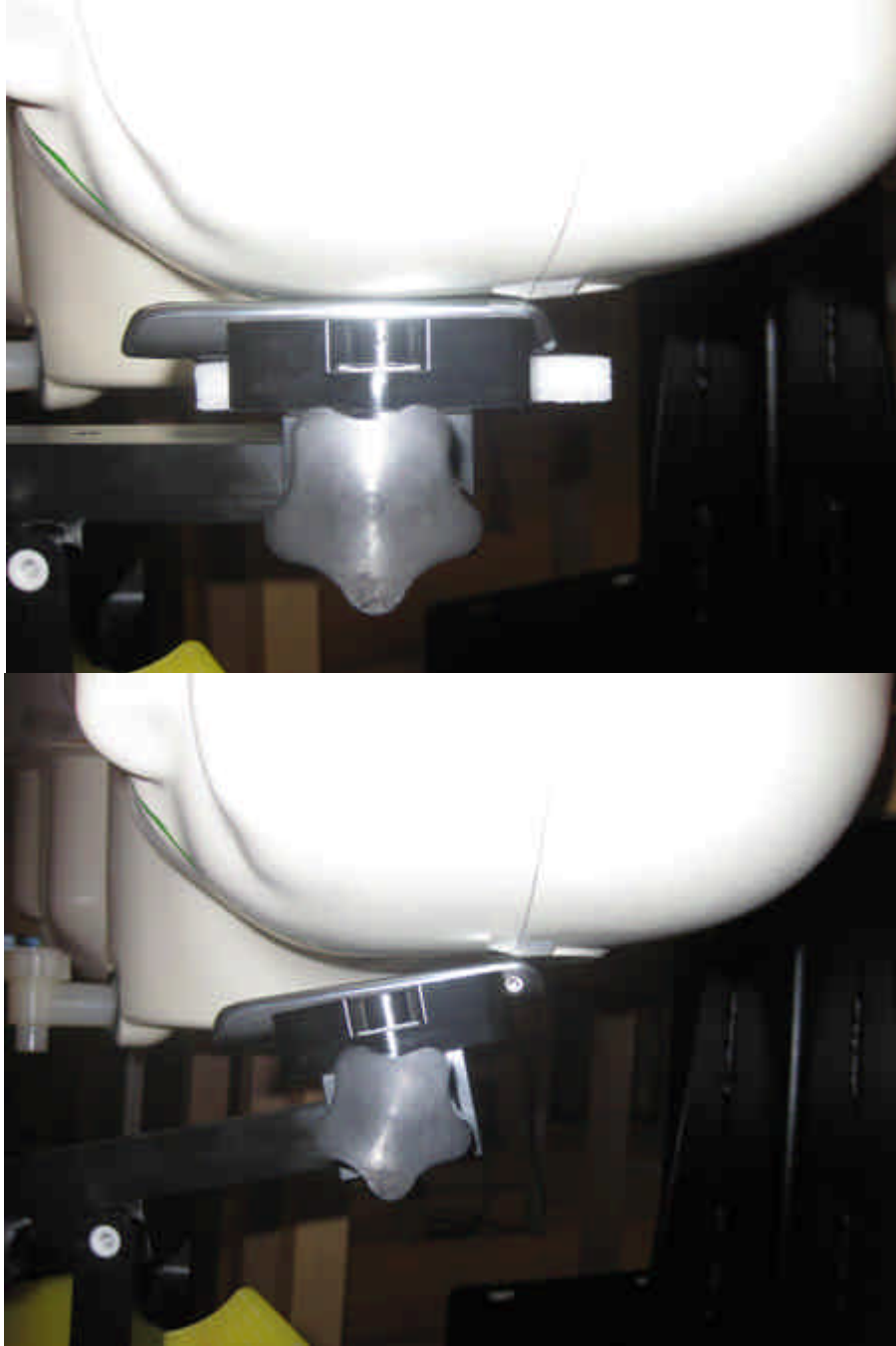
Figure E5. Head configuration (Left Touch/Tilt)
