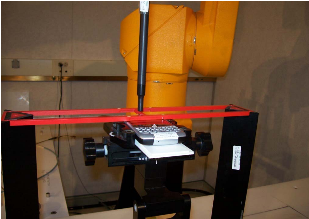
Figure 4 – HAC RF emissions test setup
