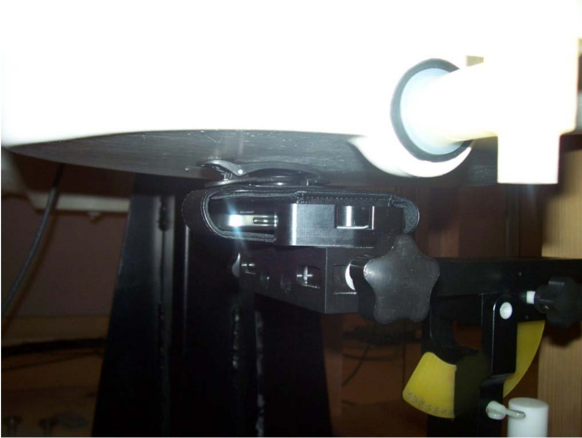
Figure E7. Body-worn configuration (Holster 2, back facing phantom)
