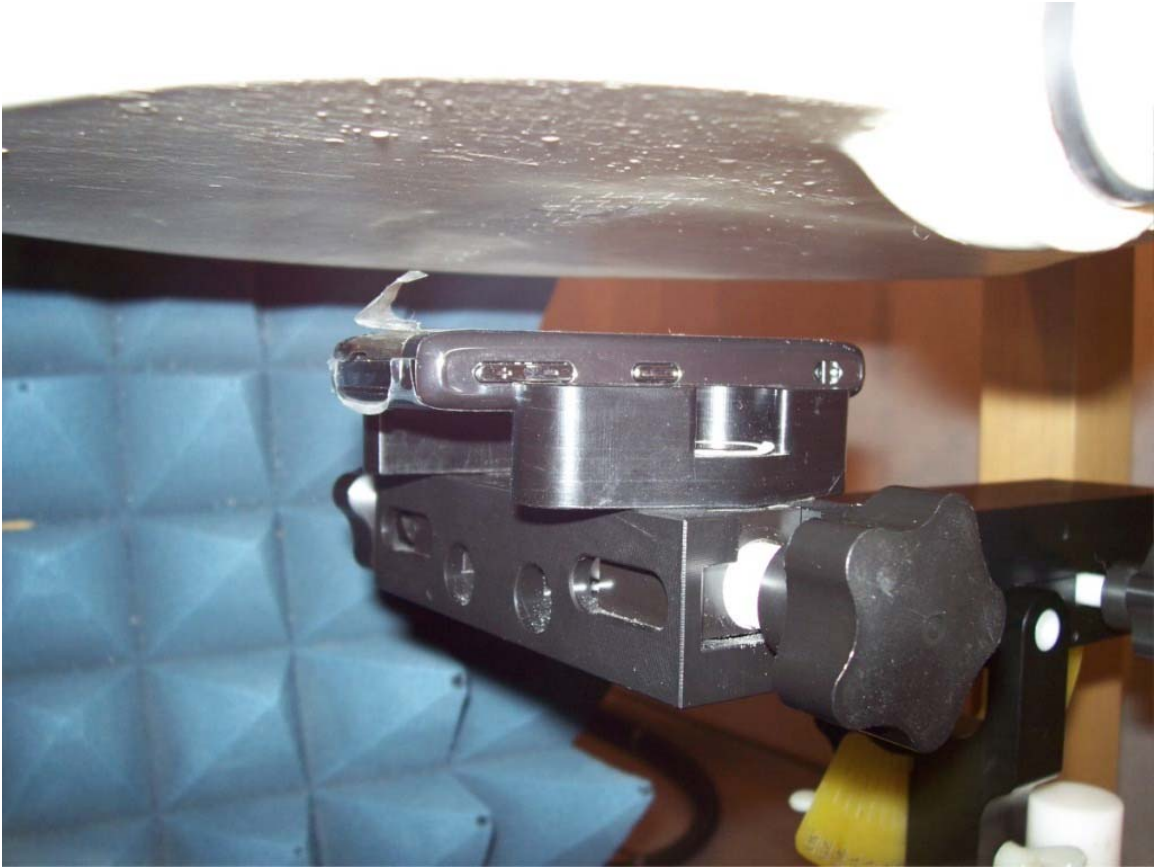
Figure E15. Body-worn configuration (No Holster, 25 mm away, back facing phantom)
