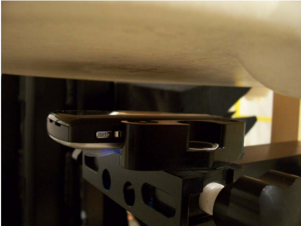
Figure E9. Body-worn configuration (No Holster, 25 mm away, back facing phantom)
