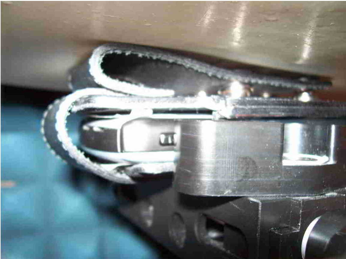
Figure E8. Body-worn configuration (Holster6, back facing phantom)
