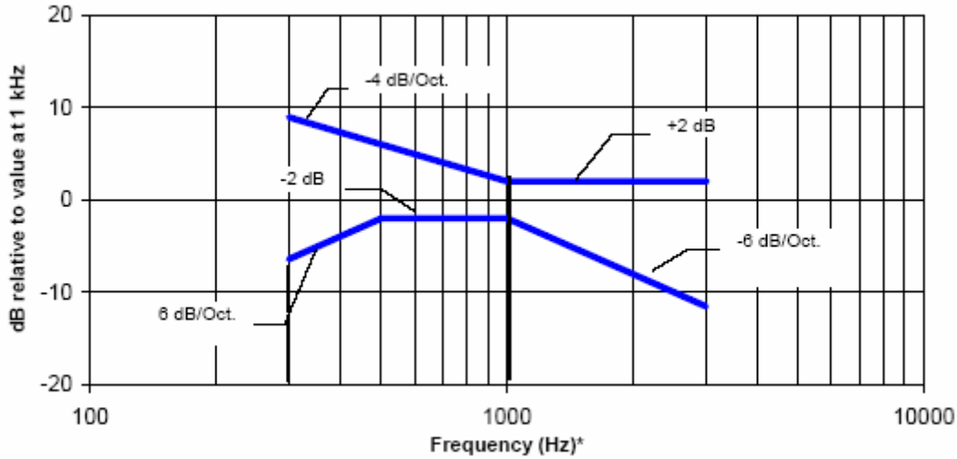
Figure 8: Magnetic field frequency response for WDs with a field between 10 dB and -13 dB (A/m) at 1 kHz
