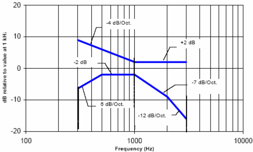
Figure 9: Magnetic field frequency response for WDs with a field that exceeds -10 dB(A/m) at 1 kHz
