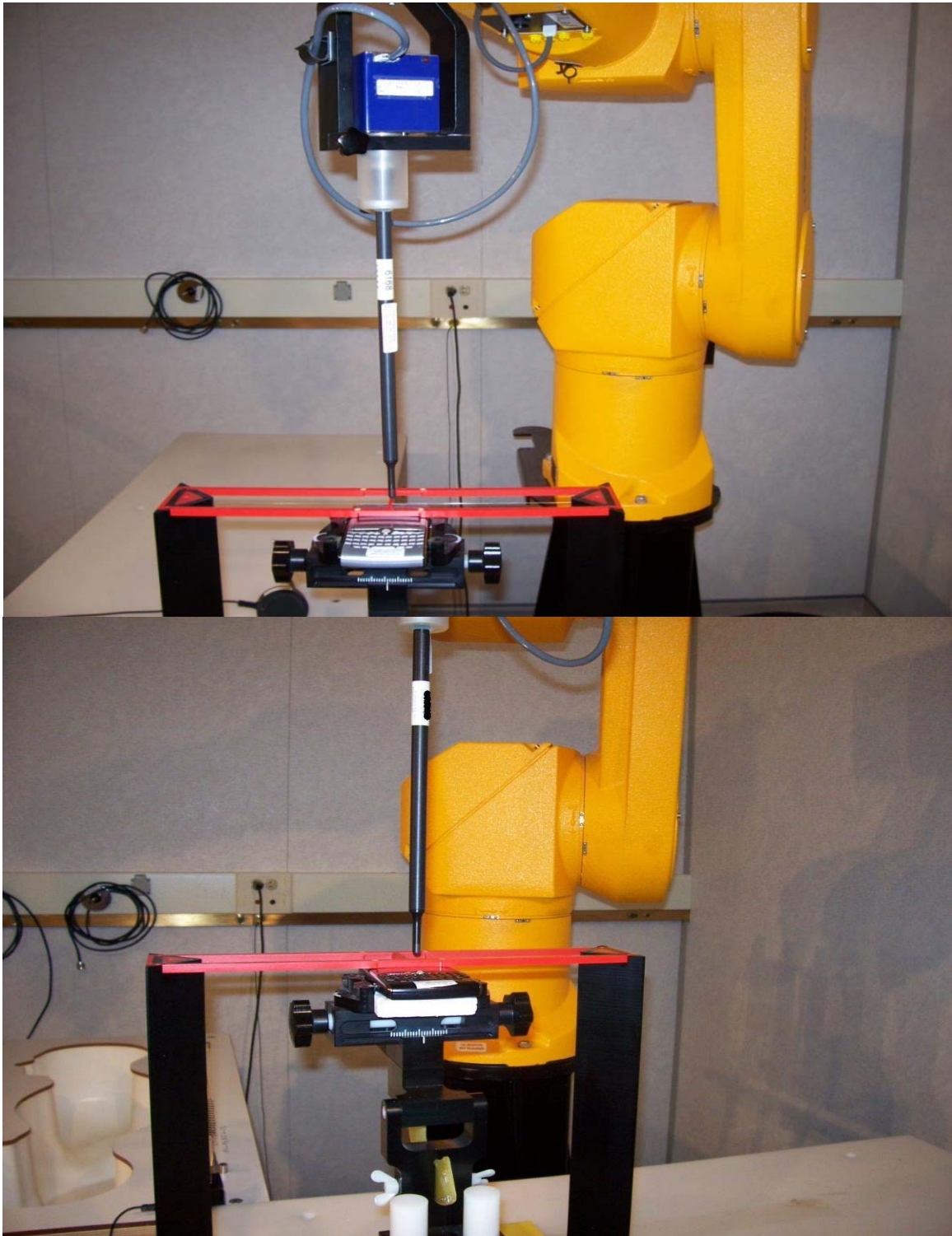
Figure 4 – HAC RF emissions test setup
