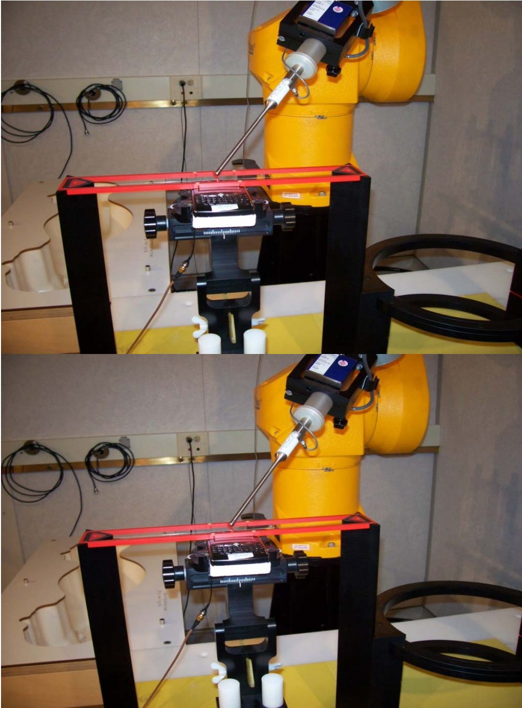
Figure E4: Audio Band Magnetic (ABM) T-Coil measurement setup
