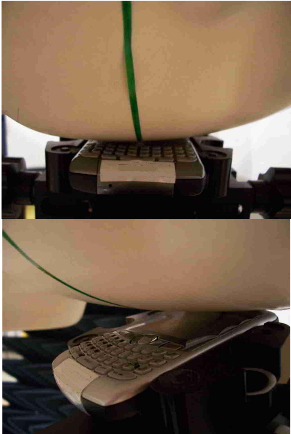
Figure E4. Head configuration (Left Touch/Tilt)
