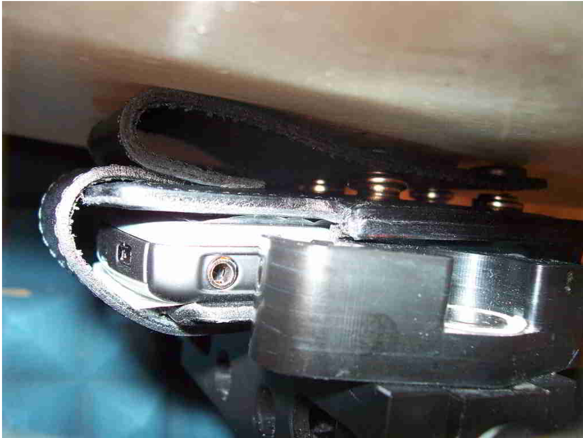
Figure E8. Body-worn configuration (Holster6, front facing phantom)
