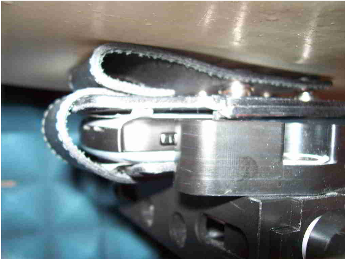
Figure E7. Body-worn configuration (Holster6, back facing phantom)
