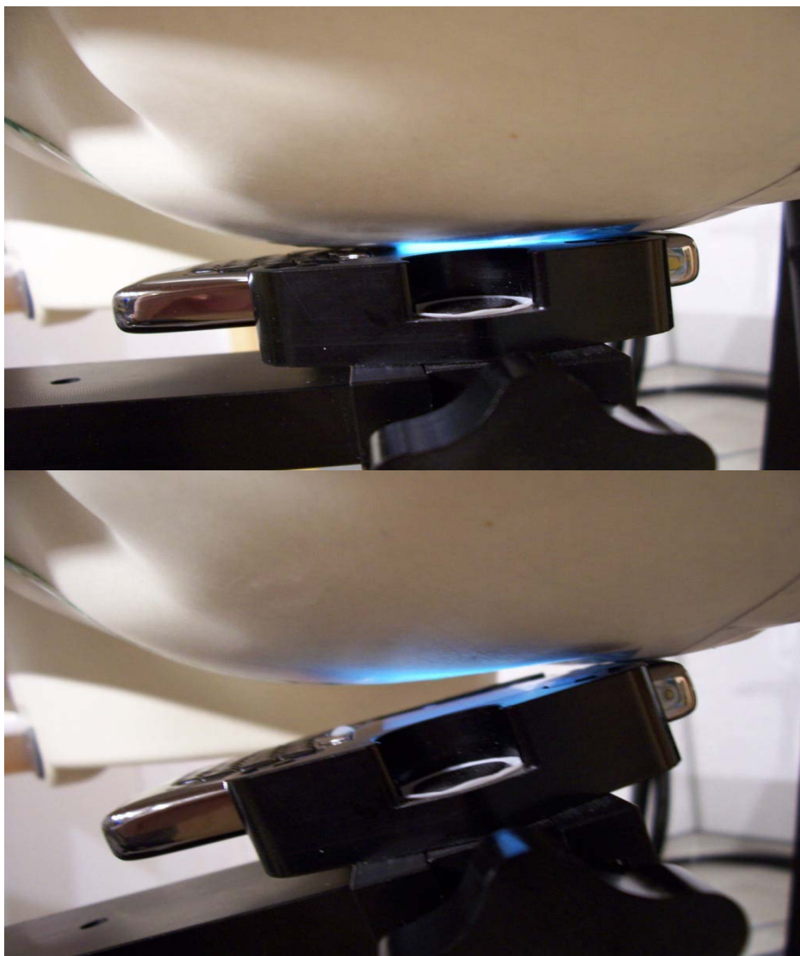
Figure E4. Head configuration (Left Touch/Tilt)
