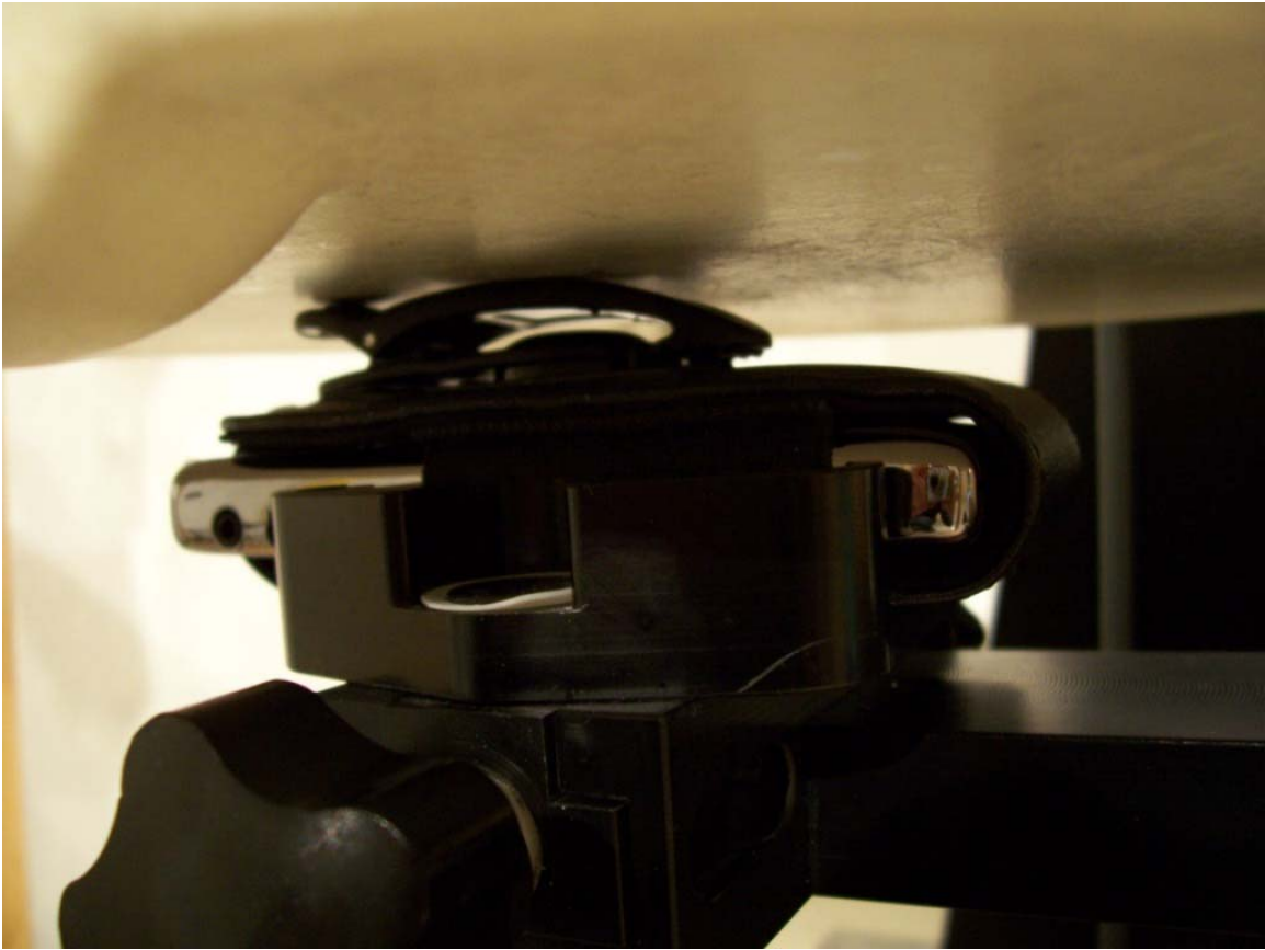
Figure E4. Body-worn configuration (Holster, front facing phantom)
