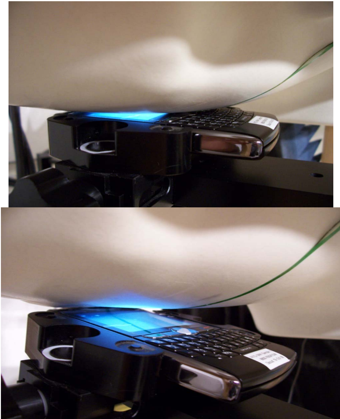
Figure E3. Head configuration (Right Touch/Tilt)
