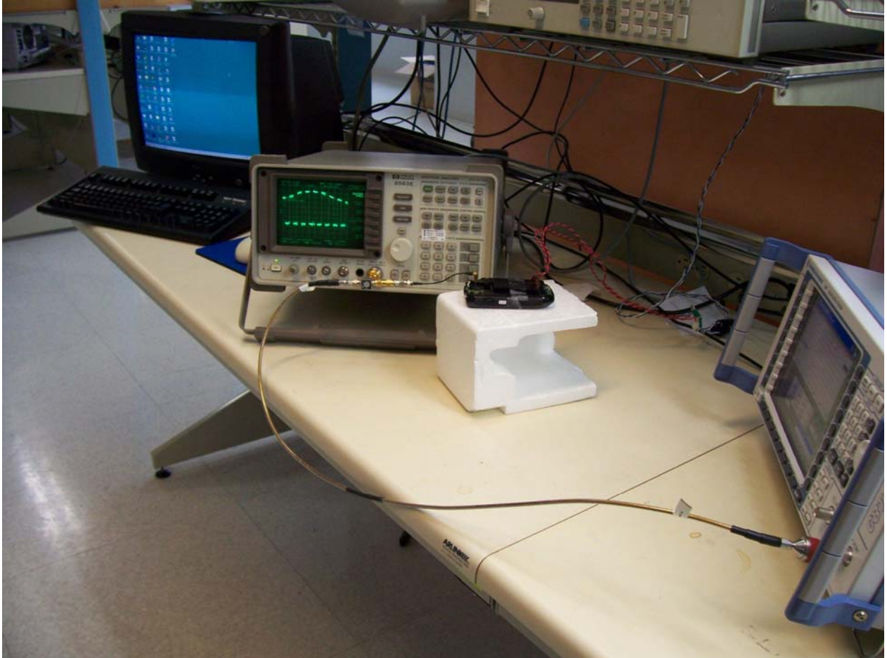
Bluetooth RF Conducted Emission Test-Setup Photo
