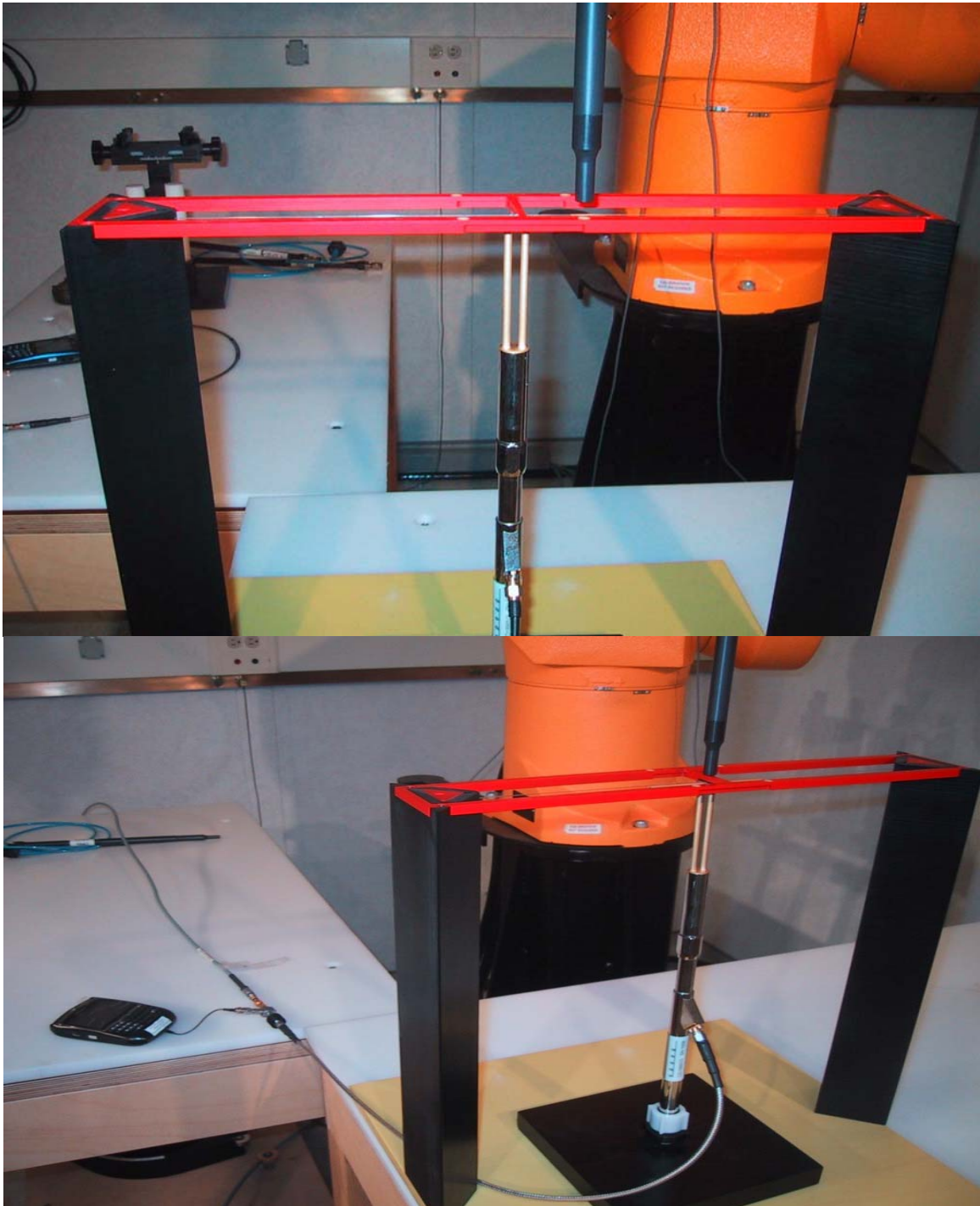
Figure 3 – PMF measurement setup
