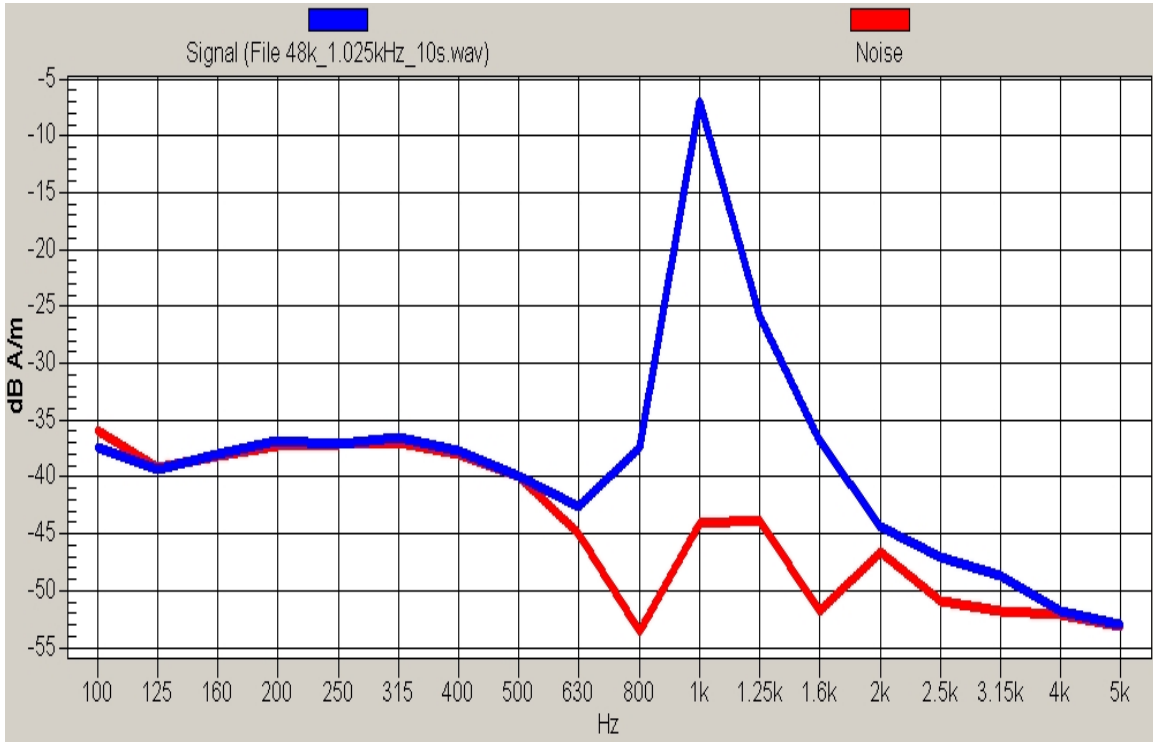
Figure A2: Reference sinusoidal 1.025 kHz signal and noise
