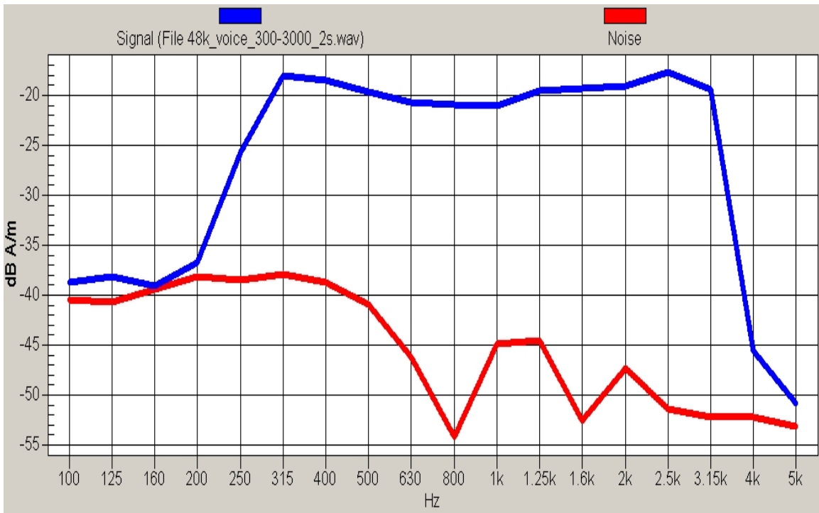
Figure A3: Reference voice simulated signal and noise
