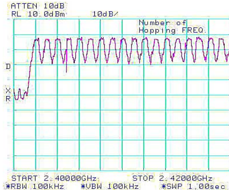
Figure 5: Number of Hopping Frequencies
