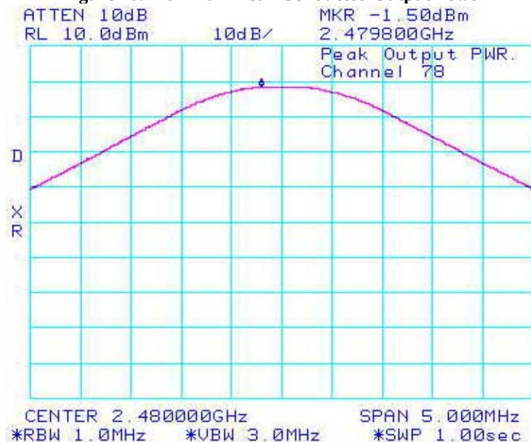
Figure 20: Maximum Peak Conducted Output Power
