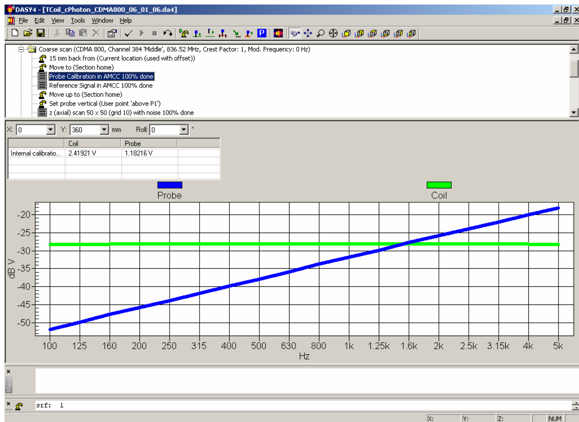
Figure 6. DASY4 ABM probe calibration
