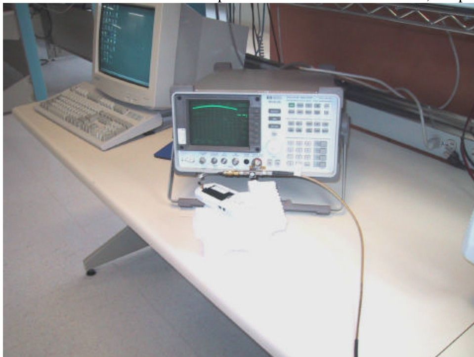
RF Bluetooth Conducted Emissions Test-Setup Photo for FCC CFR 47 Part 15, Subpart C, Class B
