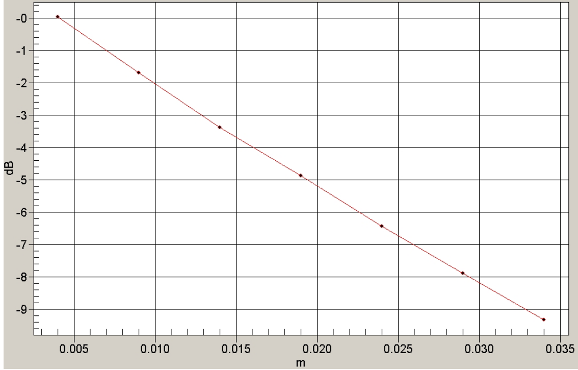
1g/10g Averaged SAR; GSM 850; Tilted left Unnamed Program/Zoom Scan/Value Along Z, X=3, Y=3 SAR
