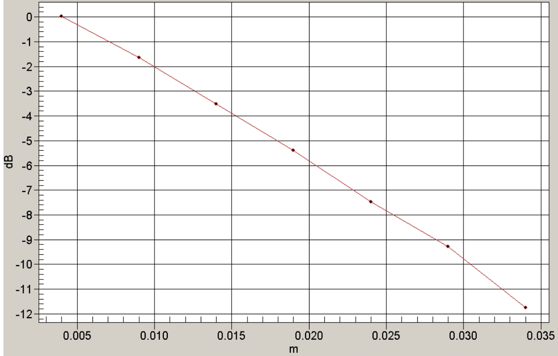
1g/10g Averaged SAR; GSM 1900; Tilted right and BT On Unnamed Program/Zoom Scan/Value Along Z, X=3, Y=3 SAR
