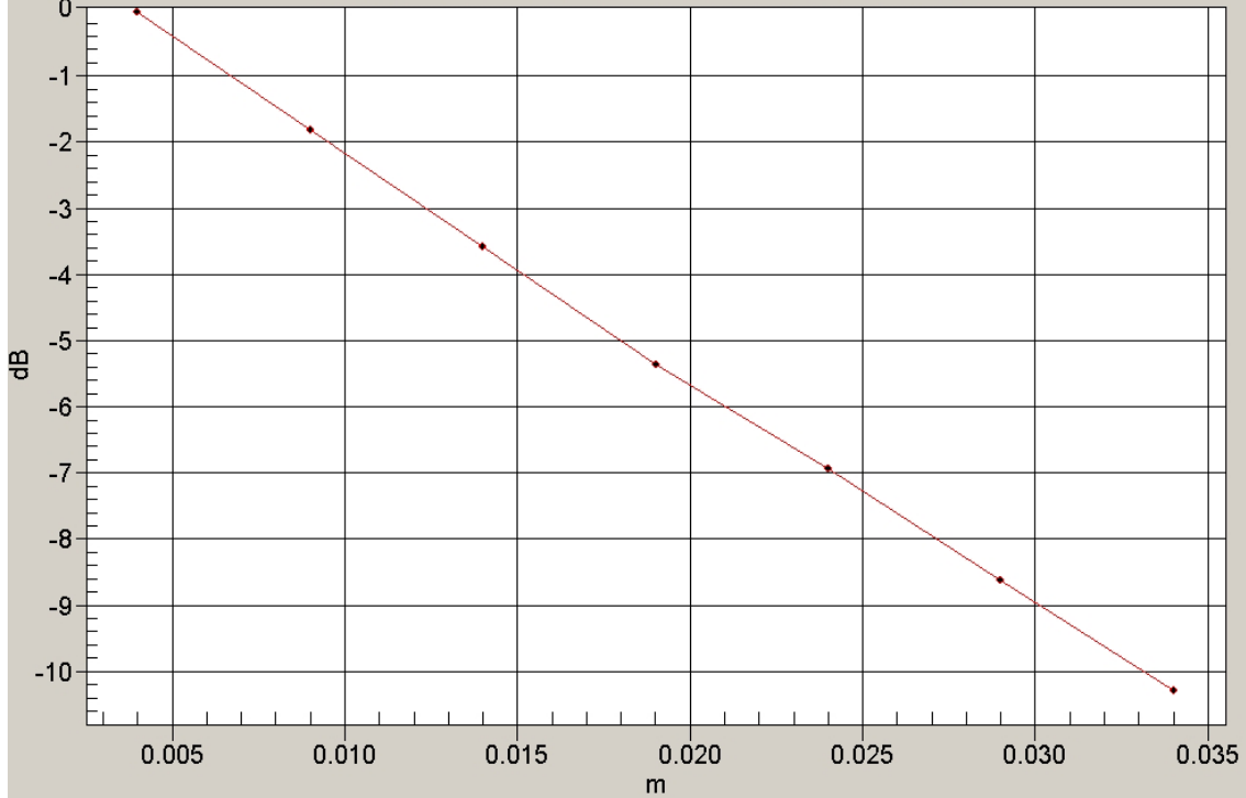
1g/10g Averaged SAR; GSM 850; Touch left with BT ON Unnamed Program/Zoom Scan/Value Along Z, X=3, Y=3 SAR
