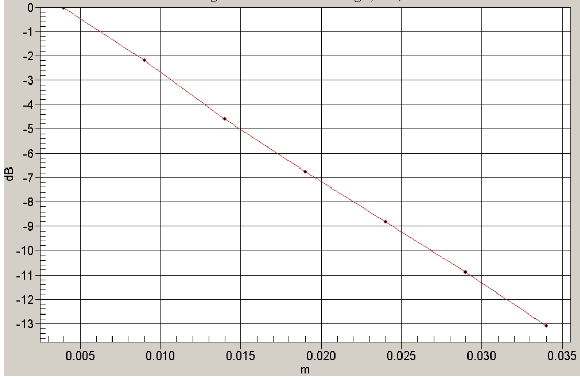
1g/10g Averaged SAR; GSM 1900; Body worn with horizontal foam holster Unnamed Program/Zoom Scan/Value Along Z, X=3, Y=3 SAR
