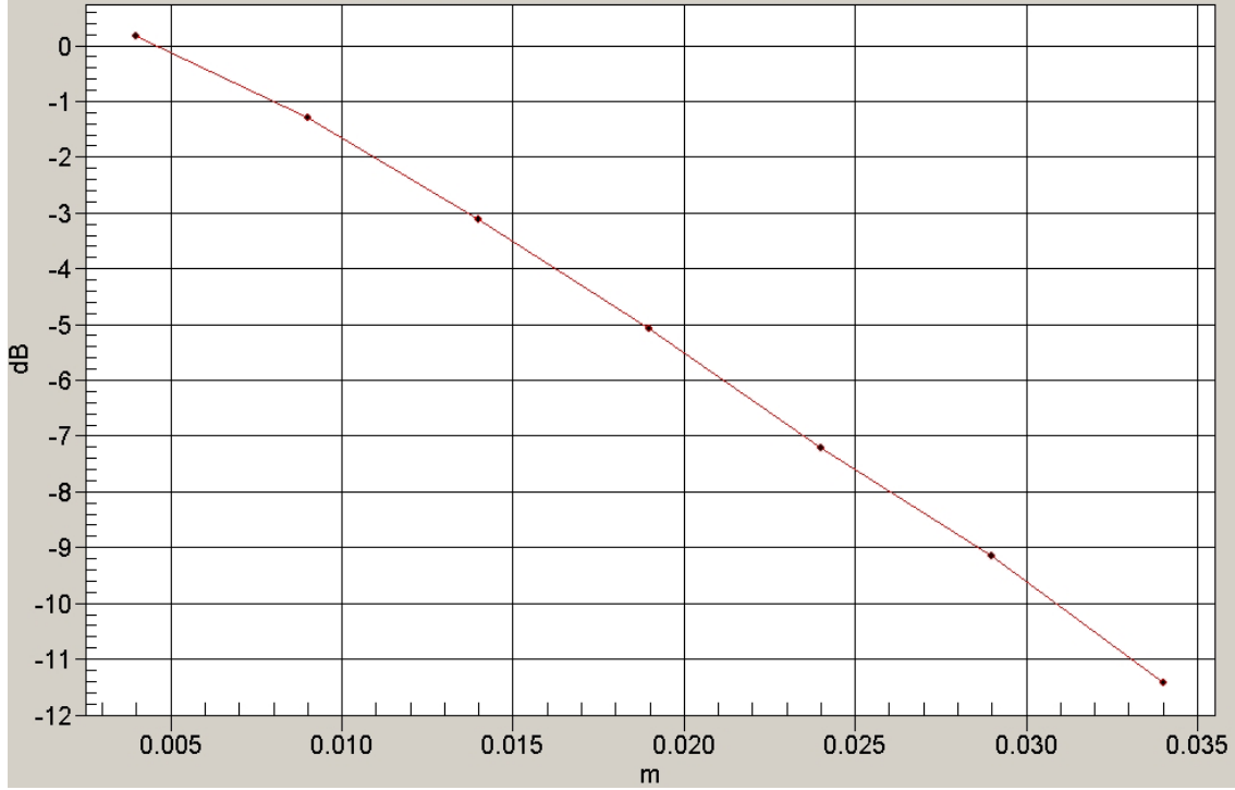
1g/10g Averaged SAR; GSM 1900; Touch left Unnamed Program/Zoom Scan/Value Along Z, X=3, Y=3 SAR
