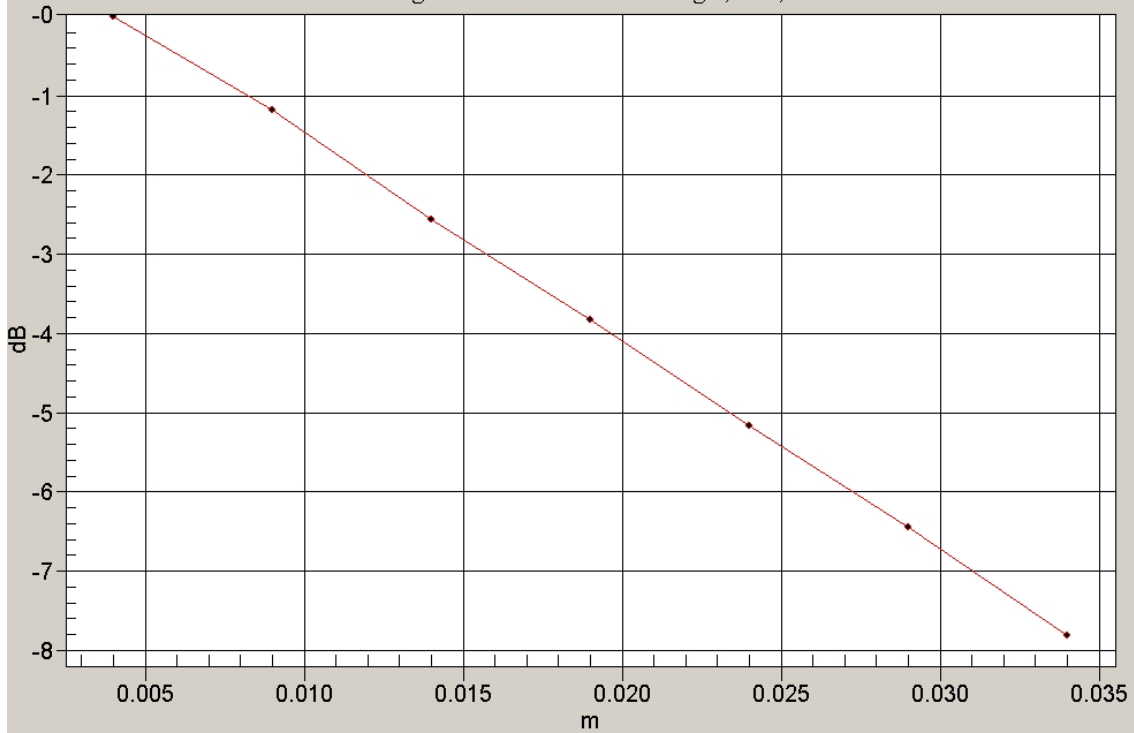
1g/10g Averaged SAR; 1900 MHz dipole validation Unnamed Program/Zoom Scan/Value Along Z, X=3, Y=3 SAR
