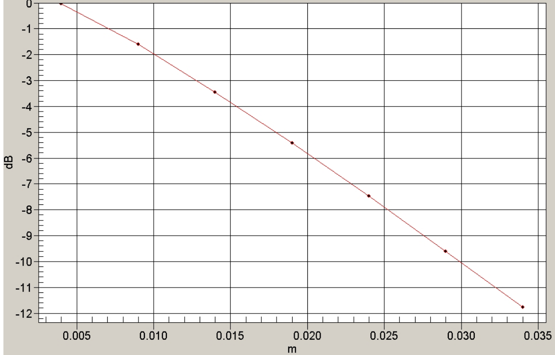
1g/10g Averaged SAR; GSM 1900; Tilted left Unnamed Program/Zoom Scan/Value Along Z, X=3, Y=3 SAR
