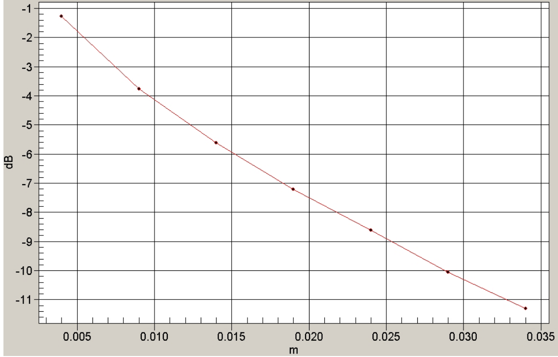
1g/10g Averaged SAR; GSM 850; Touch right Unnamed Program/Zoom Scan/Value Along Z, X=3, Y=3 SAR
