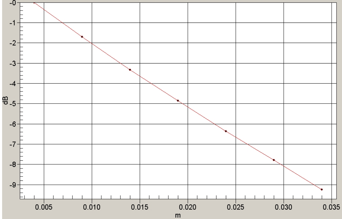
1g/10g Averaged SARGSM 850; Tilted right Unnamed Program/Zoom Scan/Value Along Z, X=3, Y=3 SAR
