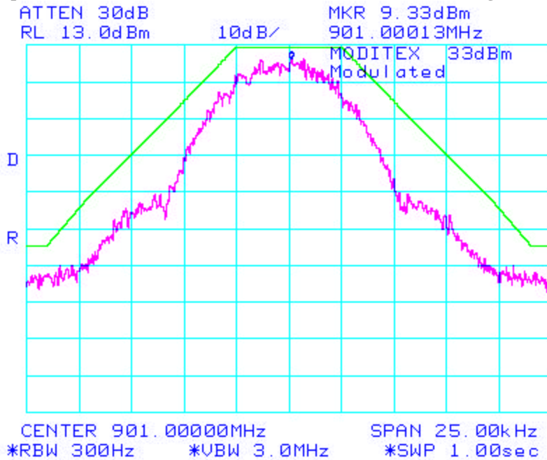
Figure 22: Occupied Bandwidth/Bandwidth Limitations, modulated Carrier, High Power, High Channel
