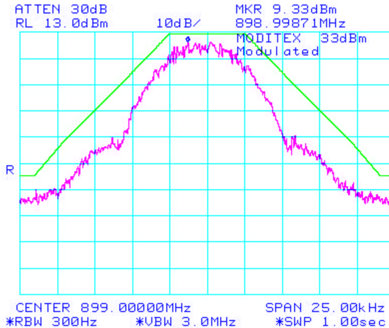
Figure 18: Occupied Bandwidth/Bandwidth Limitations, modulated Carrier, High Power, Middle Channel
