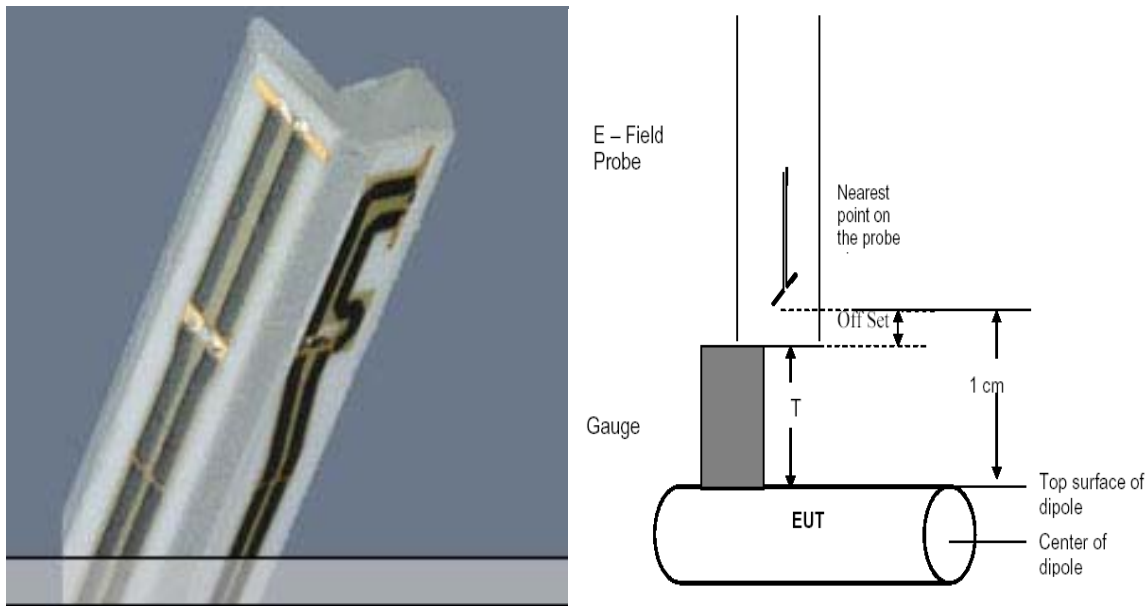
Figure 1: E-Field Probe (ER3DV6)
