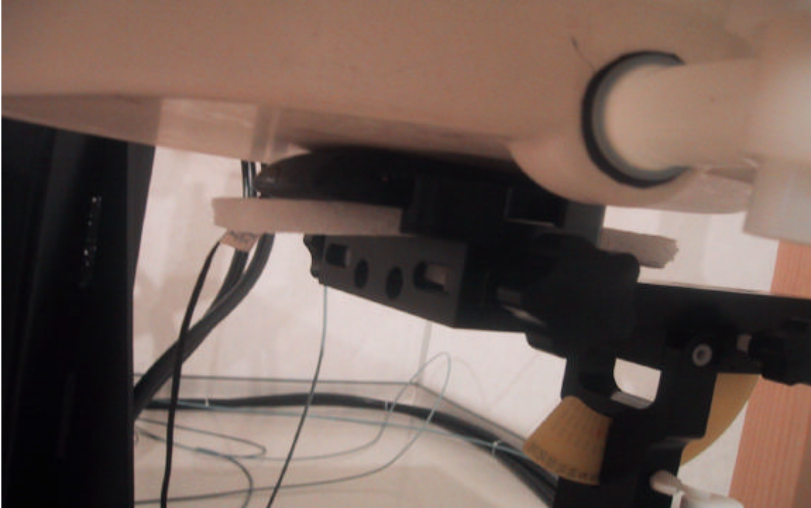
Figure E5. Hand SAR configuration, unit back touching flat phantom
