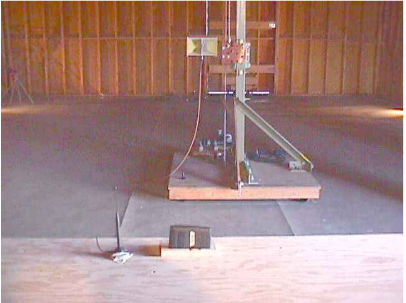
Test Configuration # 1 to 7: EUT Standalone (Side Up)
