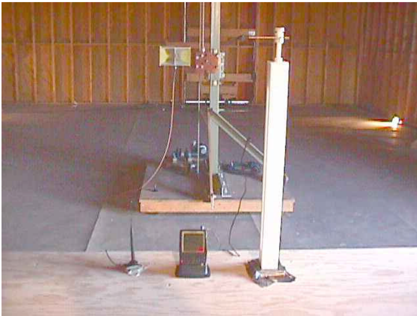
Test Configurations # 8: EUT in Cradle with Headset
