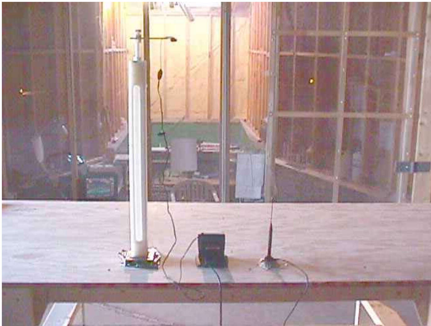
Test Configuration # 1: EUT in Cradle with Headset
