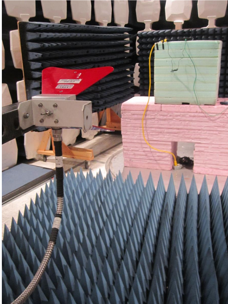
Radiated Emissions – 1 to 10 GHz
