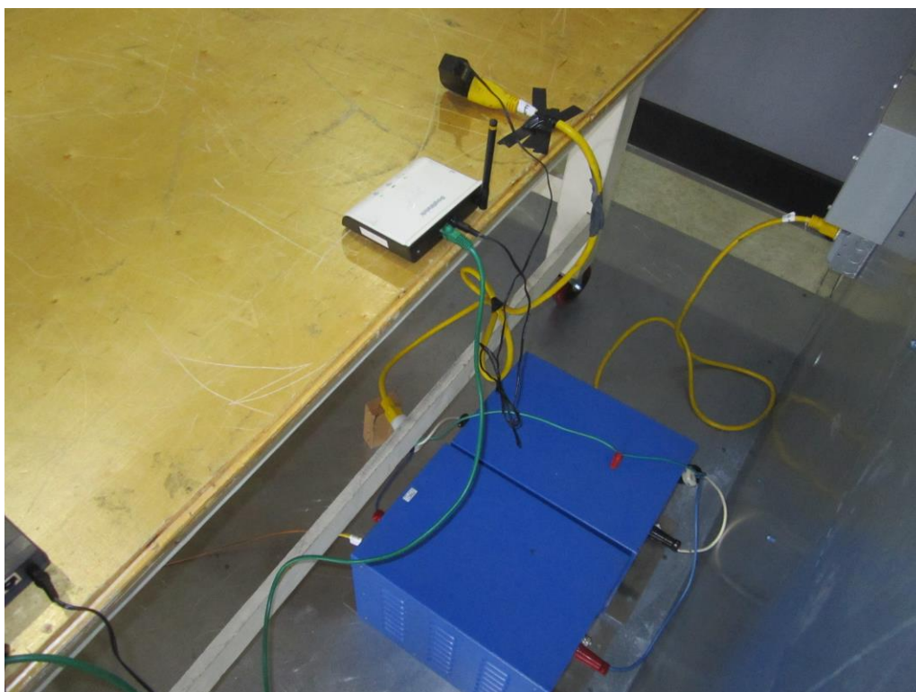
Conducted Emissions (AC Mains) – 0.15 to 30 MHz (rear)
