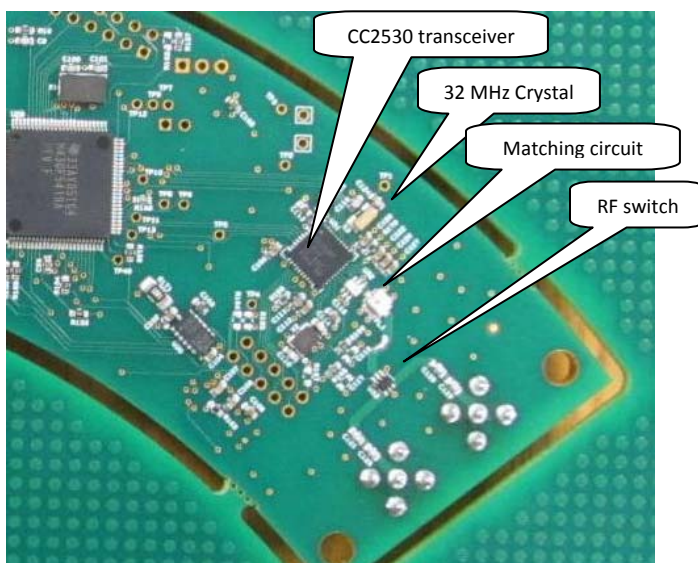
Figure 3: Close-up of radio circuitry
