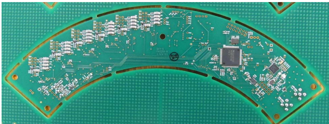
Figure 2: Bottom view of PCB-00538-10 2v3. Radio circuitry is at right.
