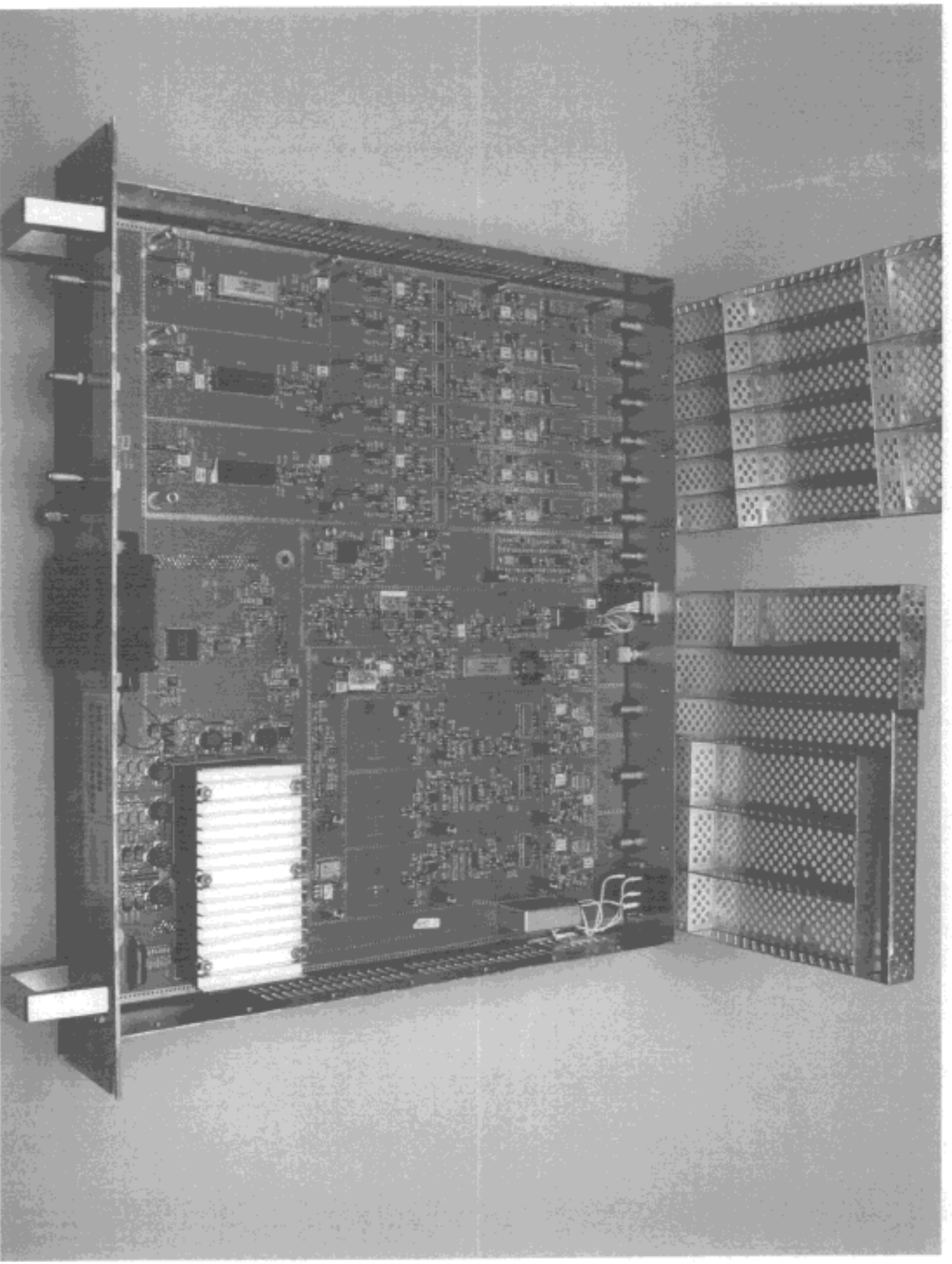
HIC, Top Cover And Top CCA Shields Removed
