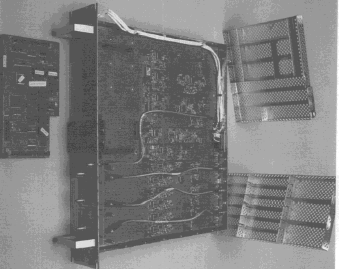
HIC, Bottom Cover And Bottom CCA Shields Removed, Daughter Card Removed
