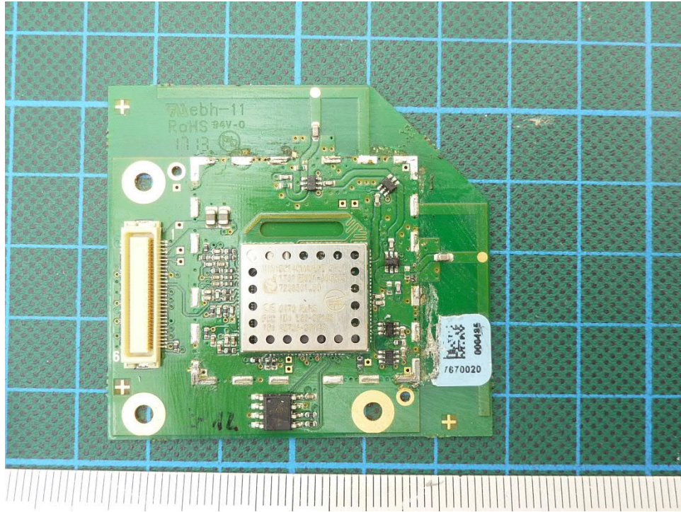
170685EUTinternal11a: DECT PCB view without shielding 2
