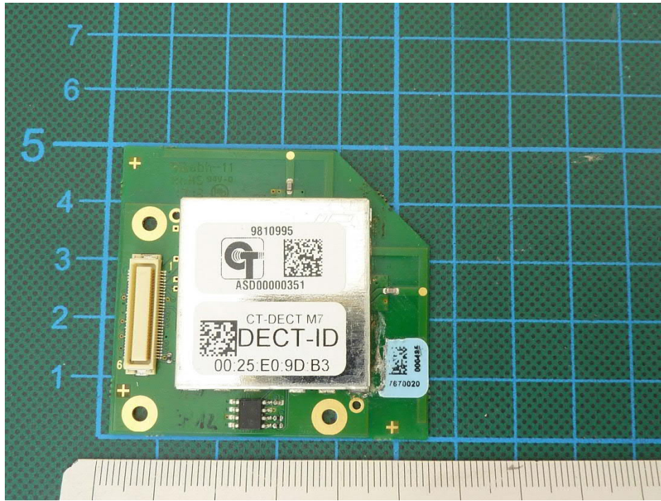
170685EUTinternal08: DECT PCB top view
