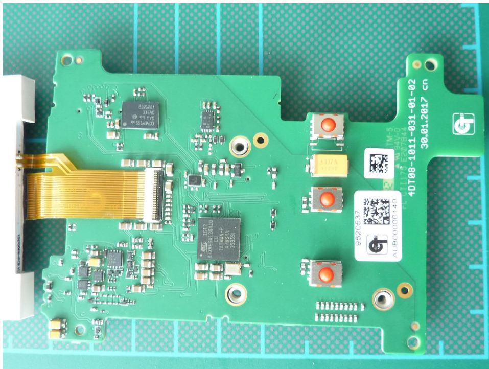
170685EUTinternal26: Main PCB bottom view 3
