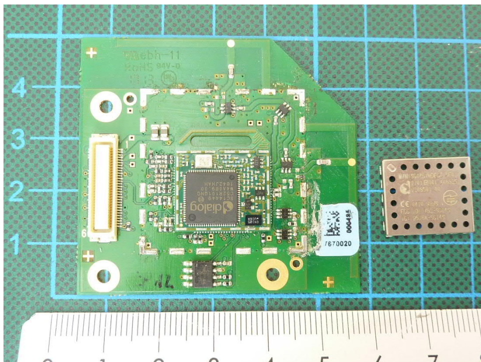
170685EUTinternal11b: DECT PCB top view without shielding 3
