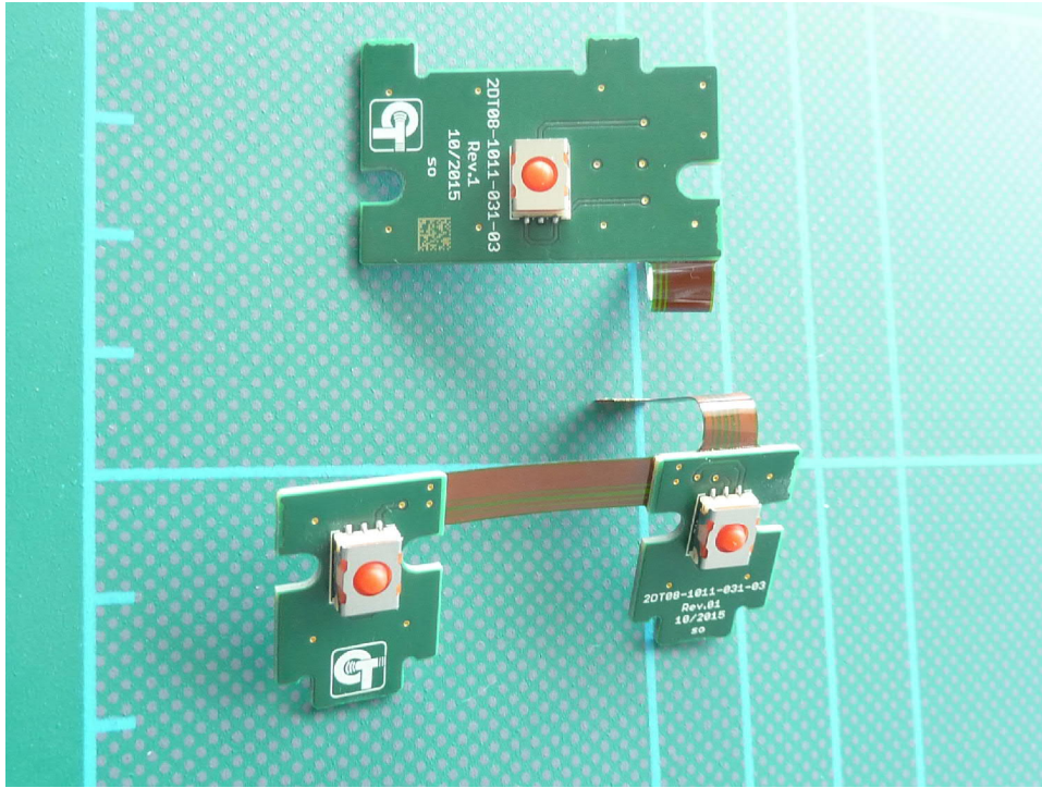
170685EUTinternal17: Side switches PCB top view 1
