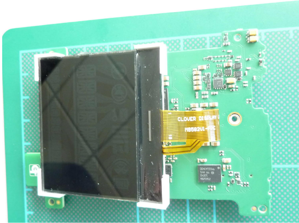
170685EUTinternal28: Main PCB bottom view 4
