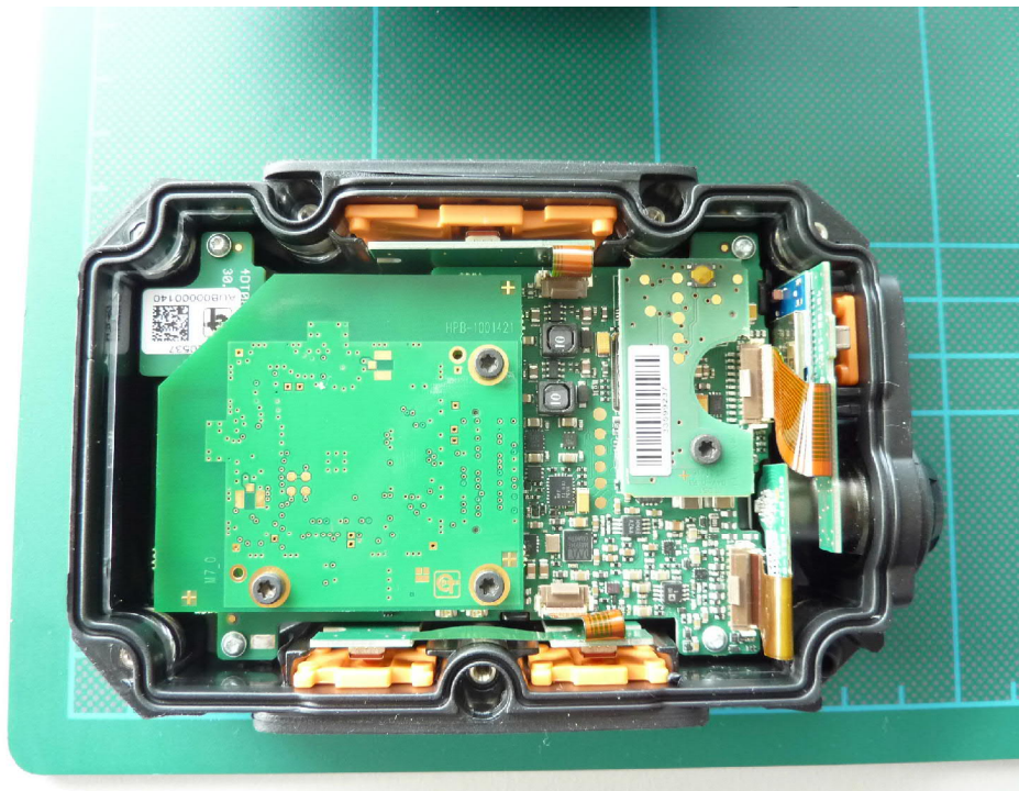
170685EUTinternal04: Inside view 2
