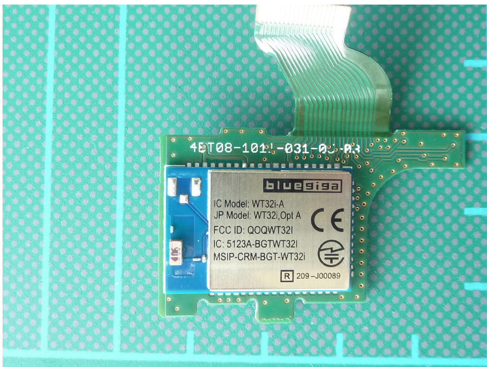
170685EUTinternal20: Bluetooth PCB top view 1
