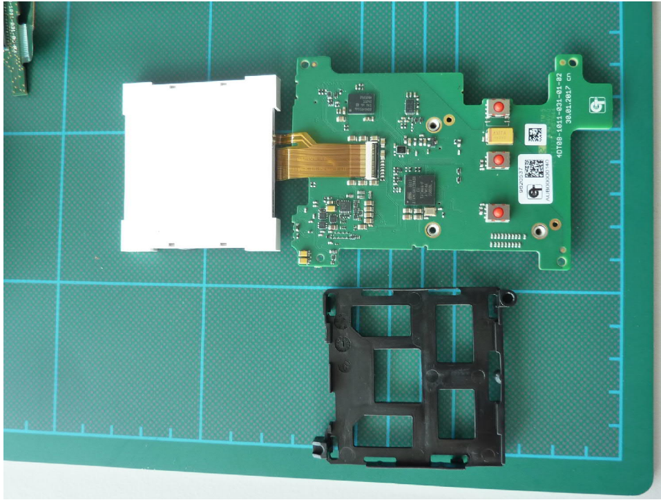
170685EUTinternal25: Main PCB bottom view 2
