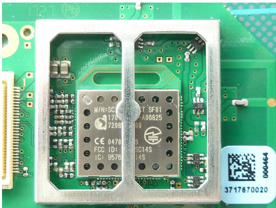
170685EUTinternal11: DECT PCB top view without shielding 1
