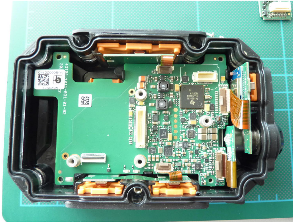
170685EUTinternal12: Inside view 6
