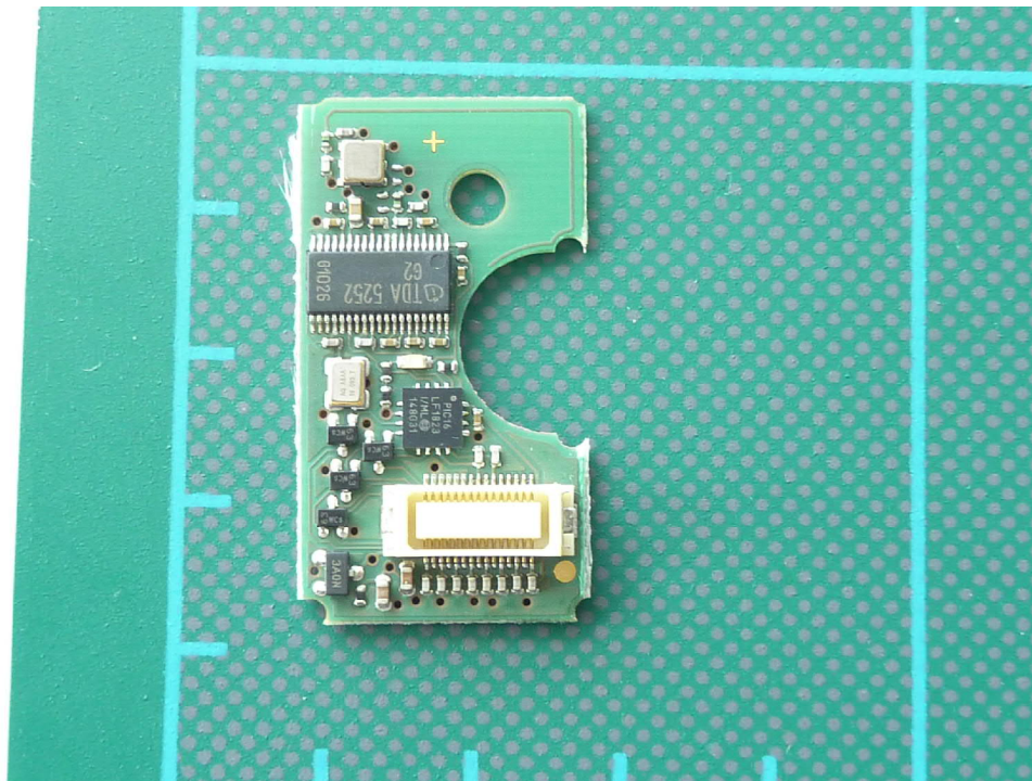
170685EUTinternal10: Sub PCB top view
