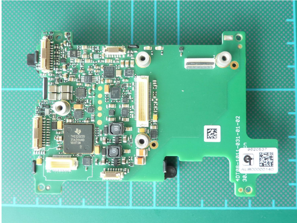
170685EUTinternal23: Main PCB top view 1
