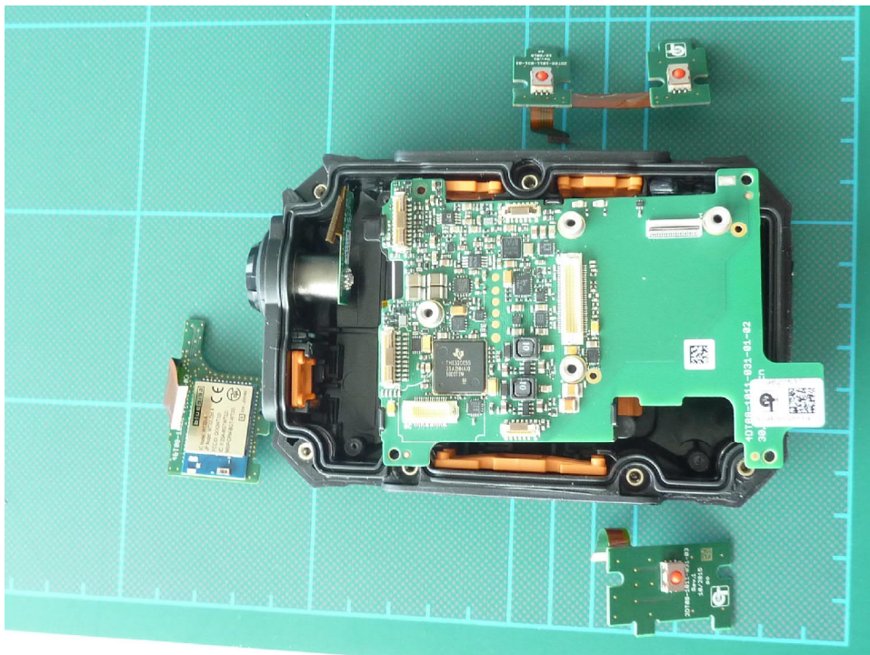
170685EUTinternal14: Inside view 7
