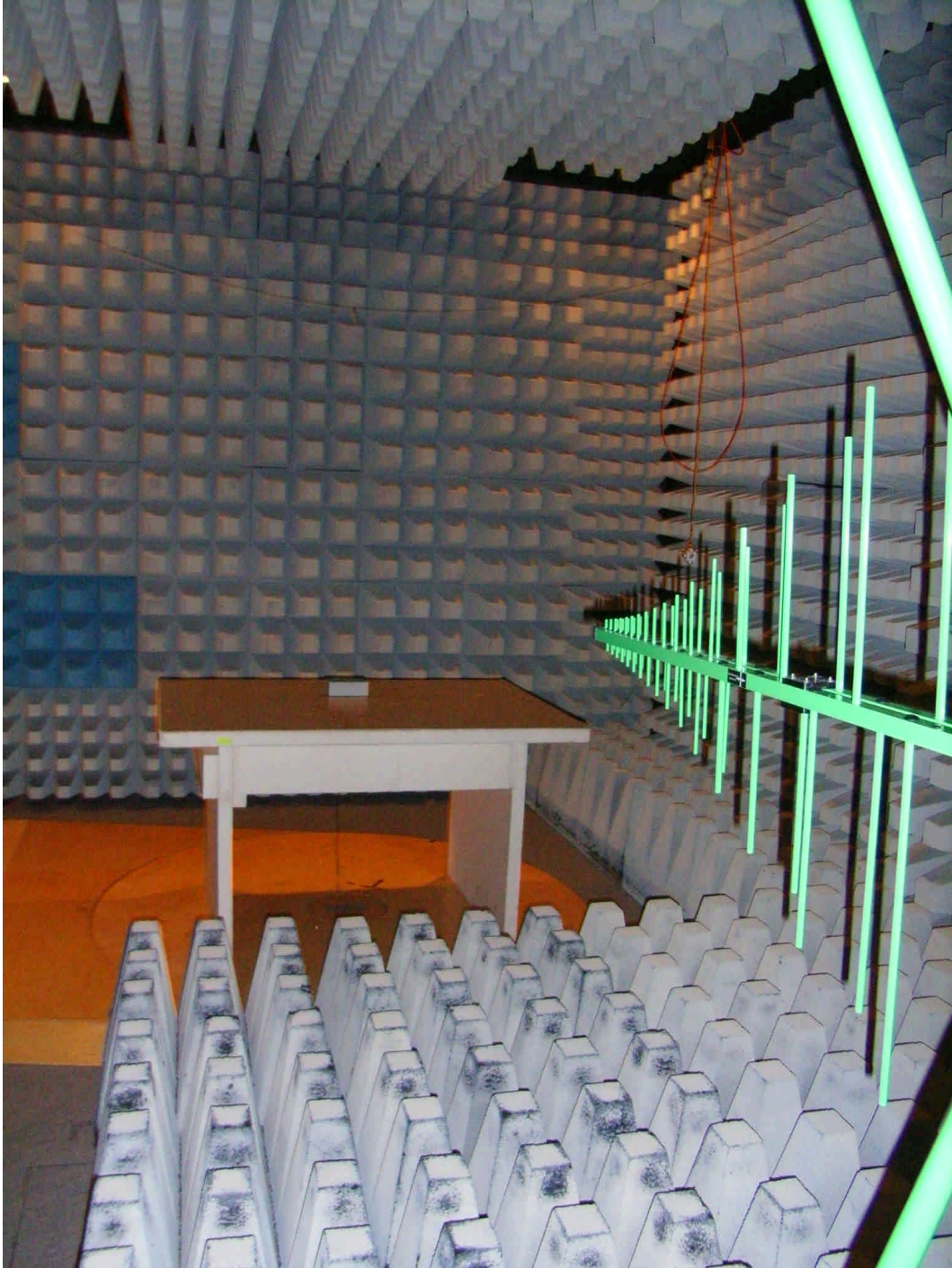
80535_EMI40.jpg Test set-up radiated emission test
