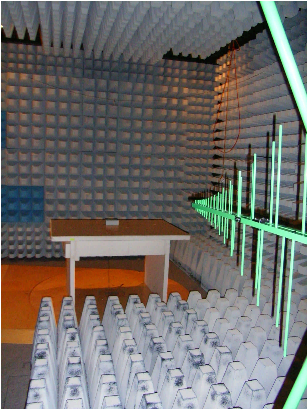
80535_EMI50.jpg Test set-up radiated emission test
