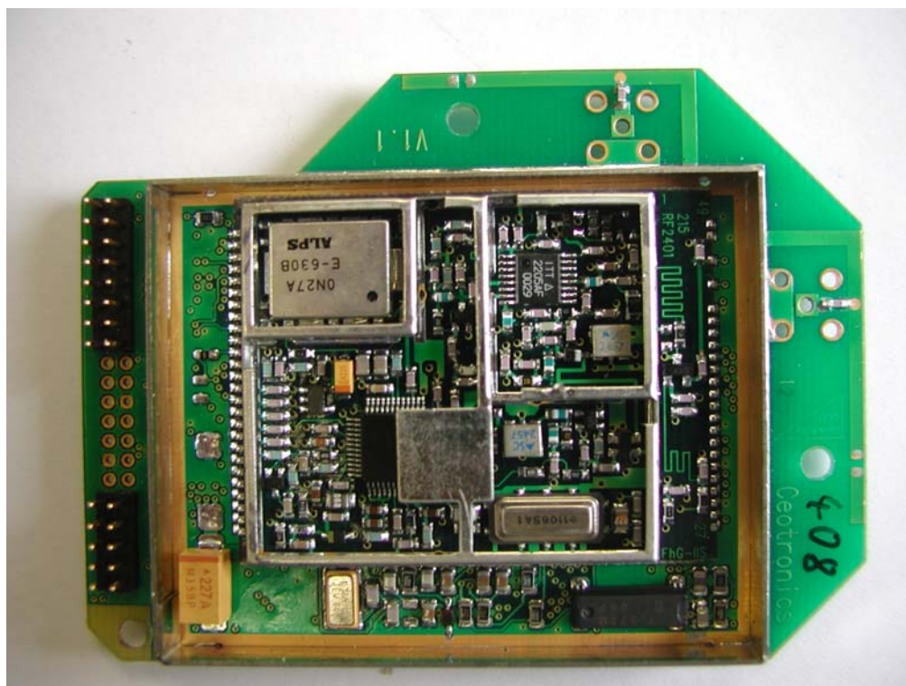
Photo 2: CT-DECT-M24 / Top View Without RF Screening Plate
