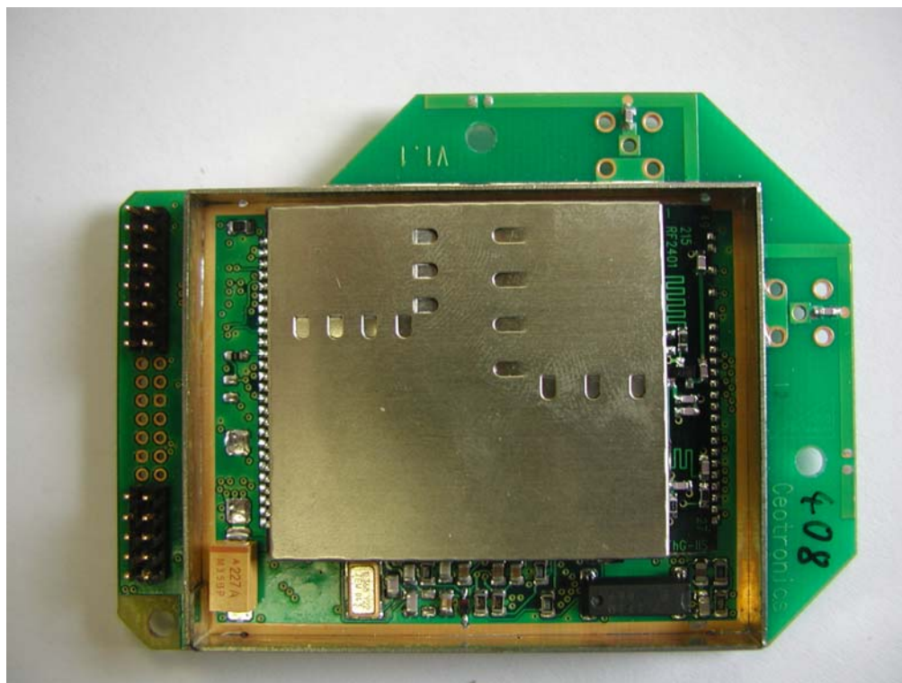
Photo 1: CT-DECT-M24 Multi / Top View Without Screening Plate
