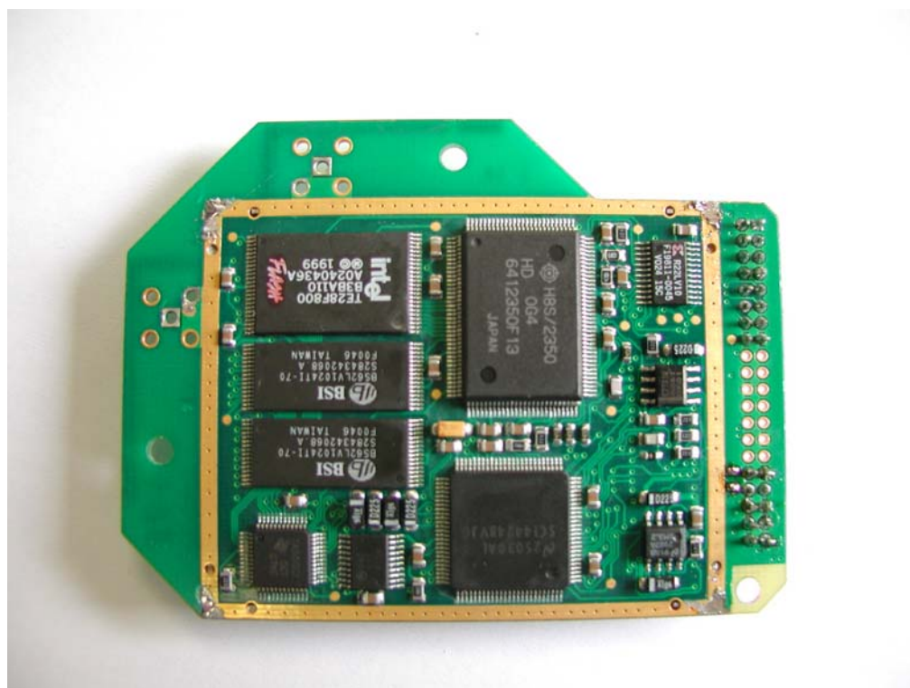
Photo 4: CT-DECT-M24 / Rear View Without Screening Plate
