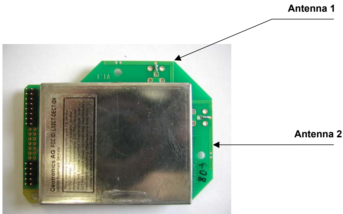
Photo 1 : Antenna Position
